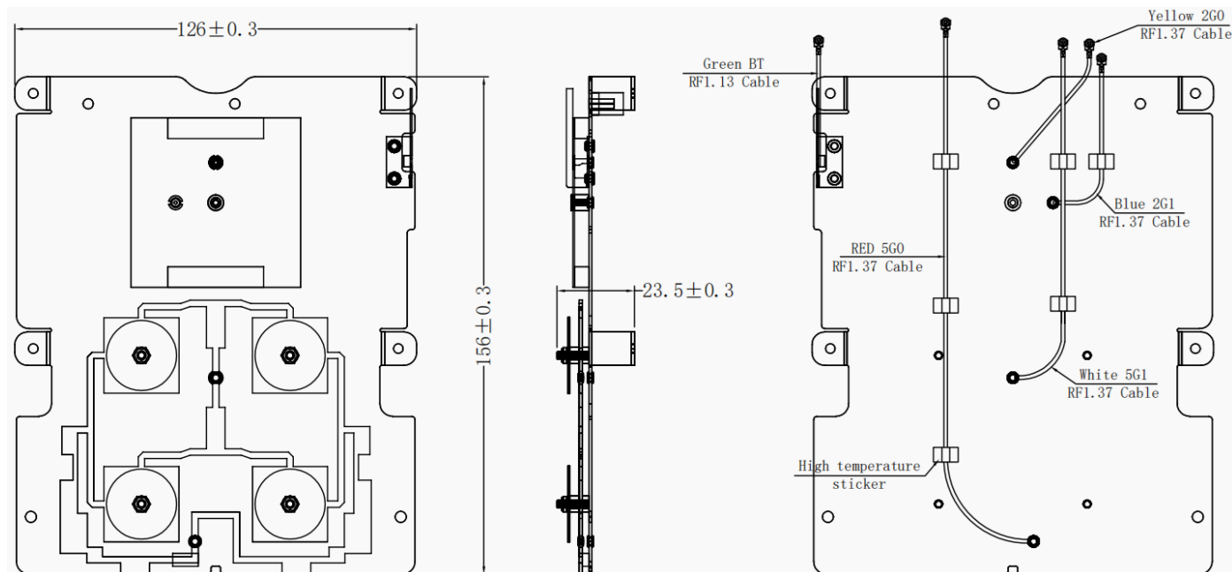
总成图 Mechanical Drawing(unit:mm)
