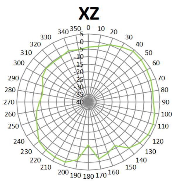
BT Antenna Radiation Patterns(unit:dB)
