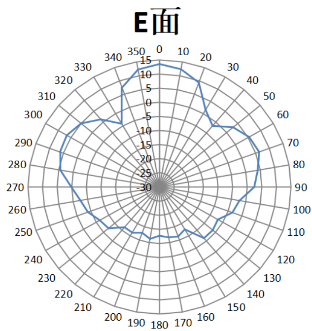
5G Antenna Radiation Patterns(unit:dB)
