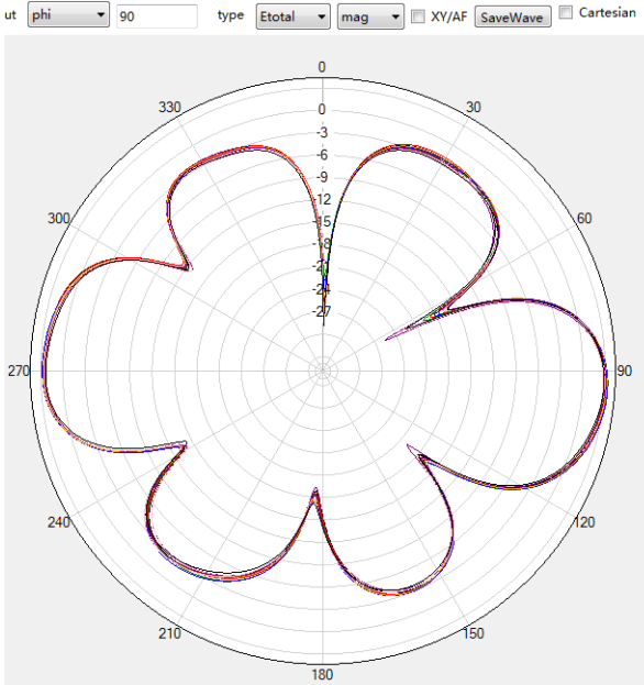
2.4G phi=90deg
