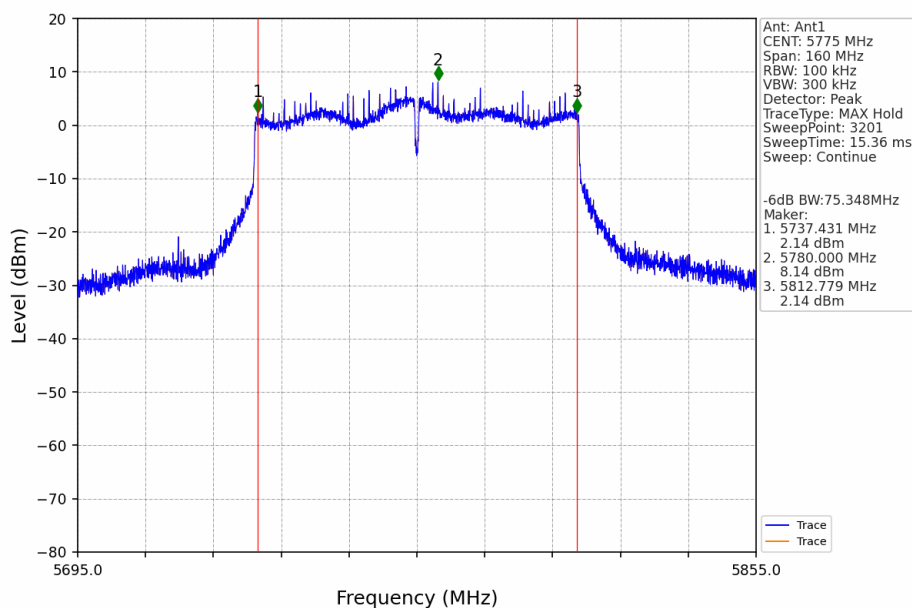
802.11ac(VHT80)_MCH_5775MHz_Ant1_NTNV
