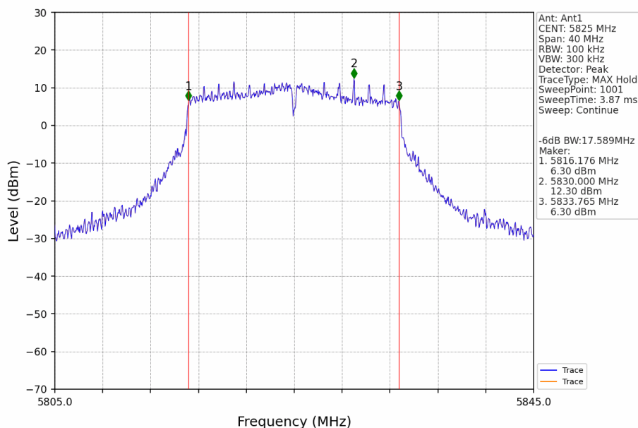
802.11ac(VHT20)_HCH_5825MHz_Ant1_NTNV
