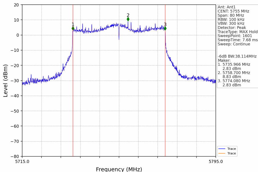
802.11ax(HEW40)_LCH_5755MHz_SU_Ant1_NTNV
