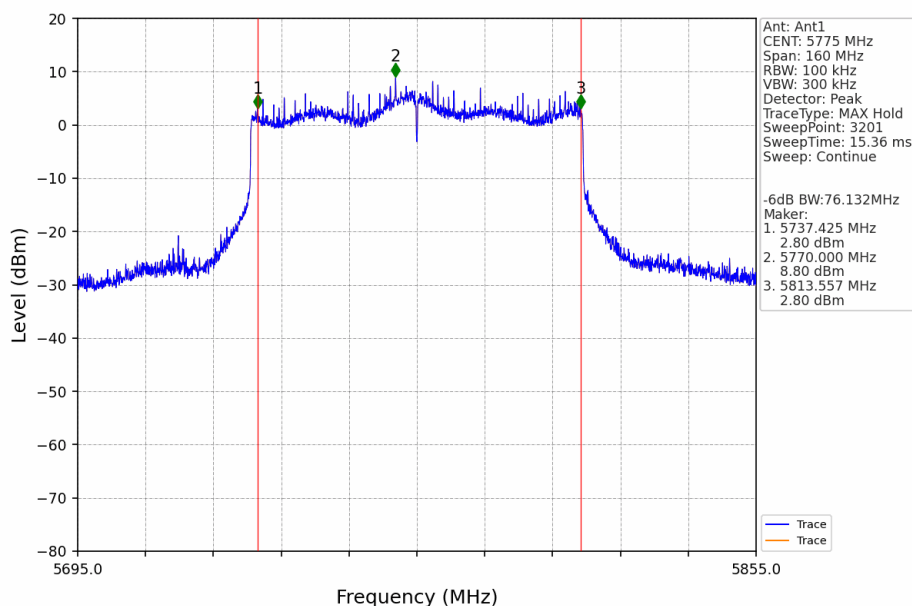
802.11ax(HEW80)_MCH_5775MHz_SU_Ant1_NTNV
