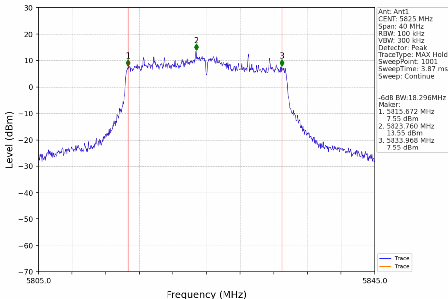
802.11ax(HEW20)_HCH_5825MHz_SU_Ant1_NTNV
