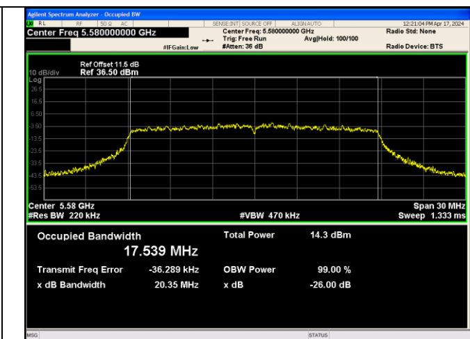
IEEE 802.11ac Channel 116 20MHz Antenna 3
