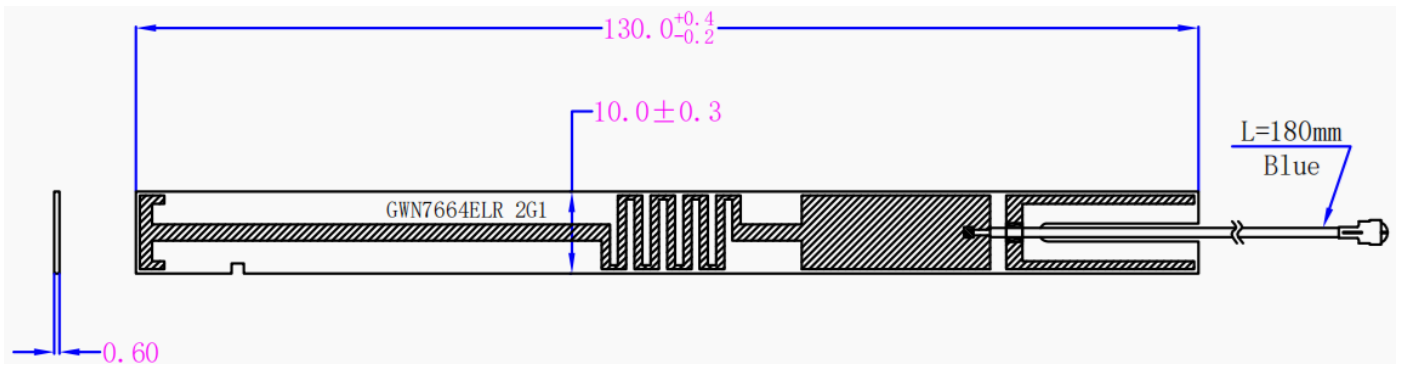
总成图 Mechanical Drawing(unit:mm)
