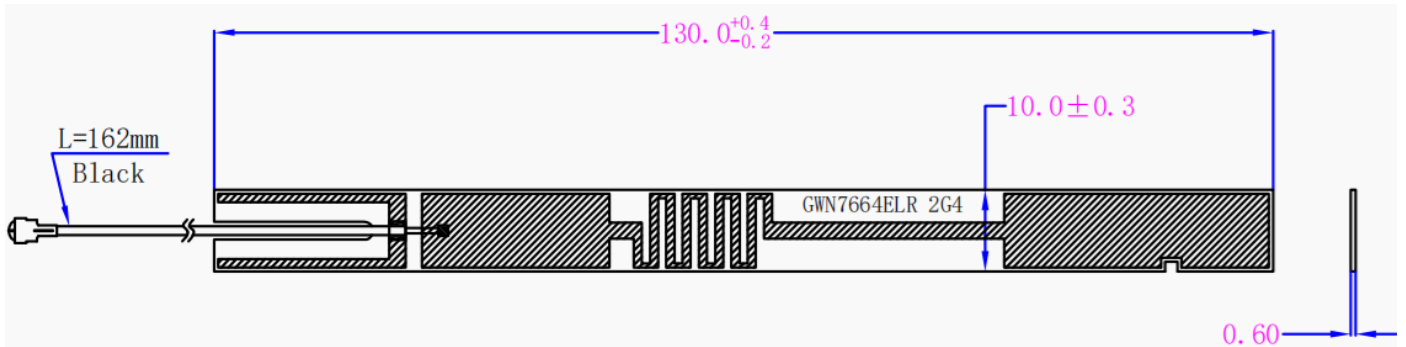
总成图 Mechanical Drawing(unit:mm)
