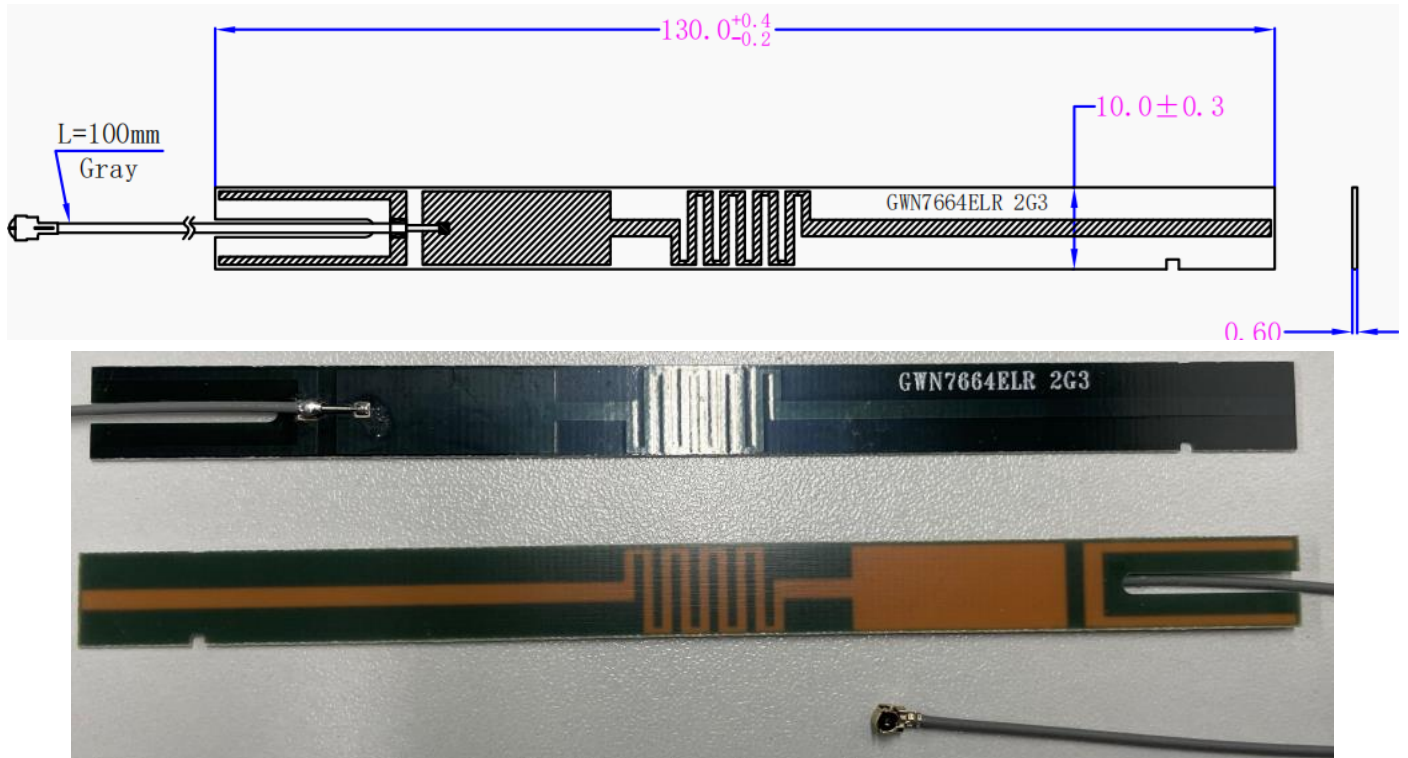
总成图 Mechanical Drawing(unit:mm)
