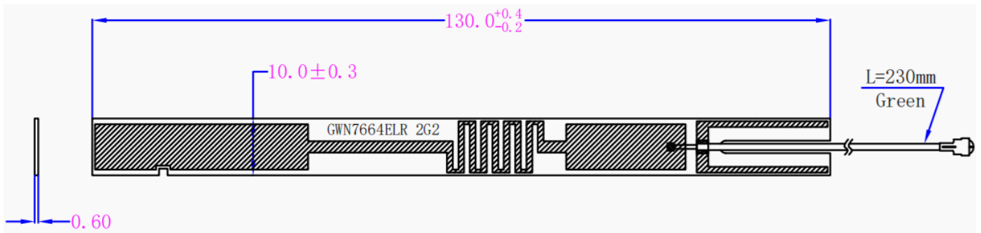
总成图 Mechanical Drawing(unit:mm)
