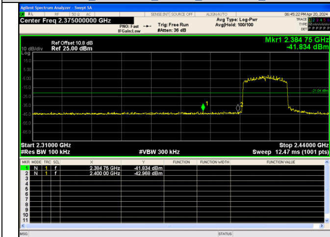
Out Of Band Emission IEEE 802.11ax Channel 1 20MHz Antenna 1 RU&Index SU
