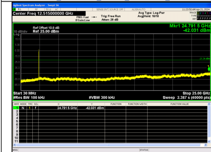
Spurious Emission IEEE 802.11ax Channel 1 20MHz Antenna 2 RU&Index SU
