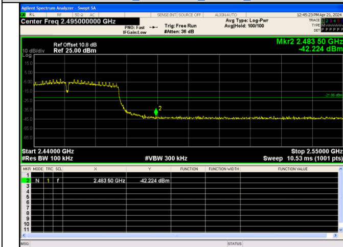
Out Of Band Emission IEEE 802.11n Channel 9 40MHz Antenna 3
