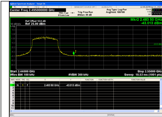
Out Of Band Emission IEEE 802.11ax_Channel 11_20MHz_Antenna 3_RU&Index SU
