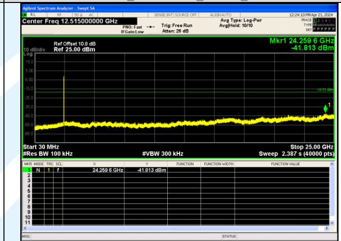
Spurious Emission IEEE 802.11n Channel 11 20MHz Antenna 3
