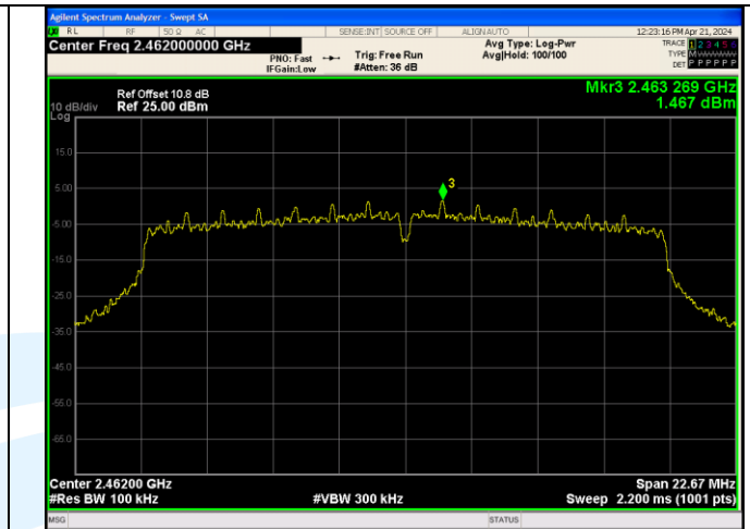
In-Band Reference Level IEEE 802.11n Channel 11 20MHz Antenna 3
