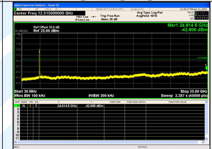
Spurious Emission IEEE 802.11n Channel 3 40MHz Antenna 3
