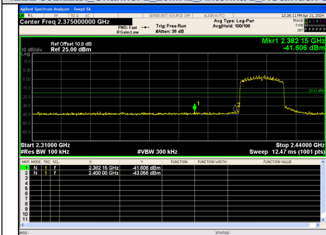
Out Of Band Emission IEEE 802.11ax Channel 1 20MHz Antenna 3 RU&Index SU
