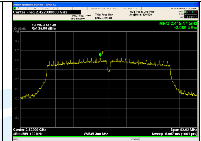
In-Band Reference Level IEEE 802.11n Channel 3 40MHz Antenna 3
