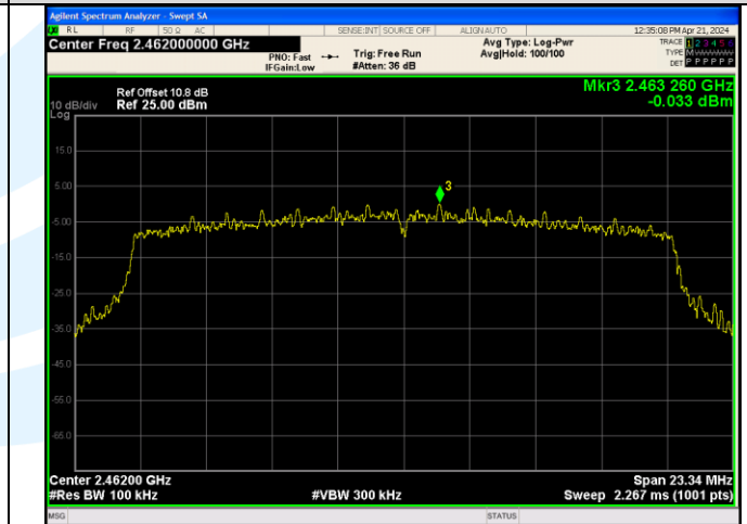
In-Band Reference Level IEEE 802.11ax_Channel 11_20MHz_Antenna 3_RU&Index SU
