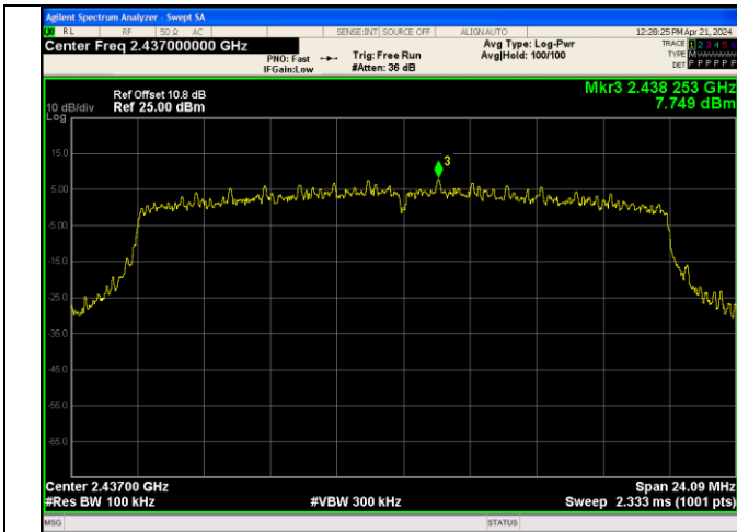
In-Band Reference Level IEEE 802.11ax Channel 6 20MHz Antenna 3 RU&Index SU
