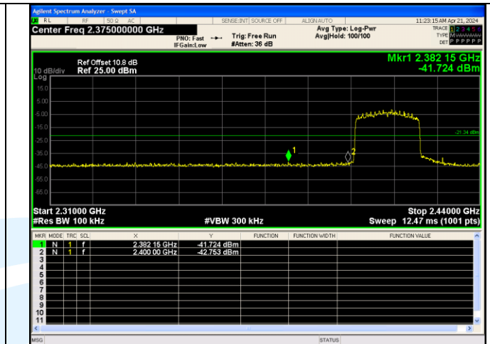
Out Of Band Emission IEEE 802.11ax Channel 1 20MHz Antenna 2 RU&Index SU
