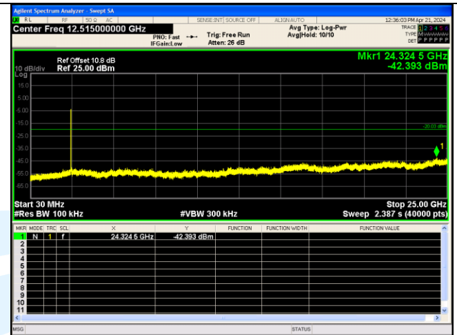
Spurious Emission IEEE 802.11ax_Channel 11_20MHz_Antenna 3_RU&Index SU
