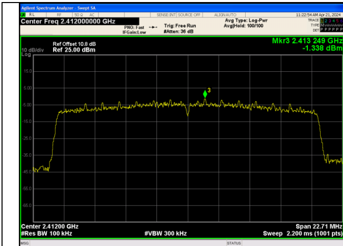
In-Band Reference Level IEEE 802.11ax Channel 1 20MHz Antenna 2 RU&Index SU
