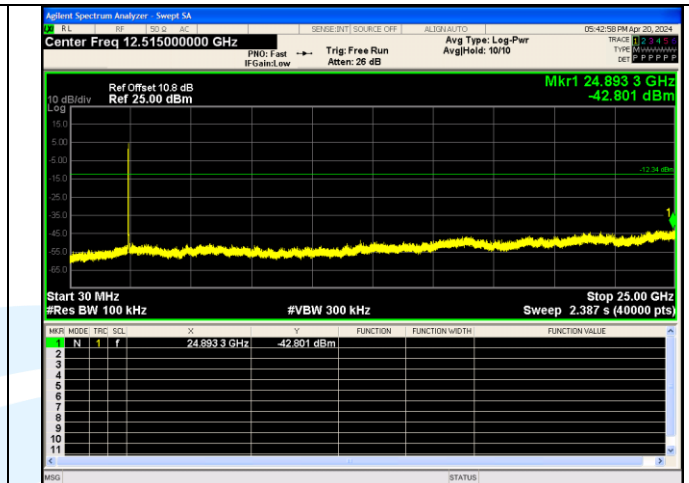
Spurious Emissions IEEE 802.11ax Channel 6 20MHz Antenna 0 RU&Index SU
