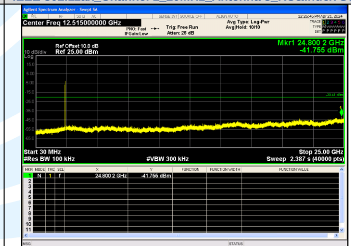
Spurious Emission IEEE 802.11ax Channel 1 20MHz Antenna 3 RU&Index SU
