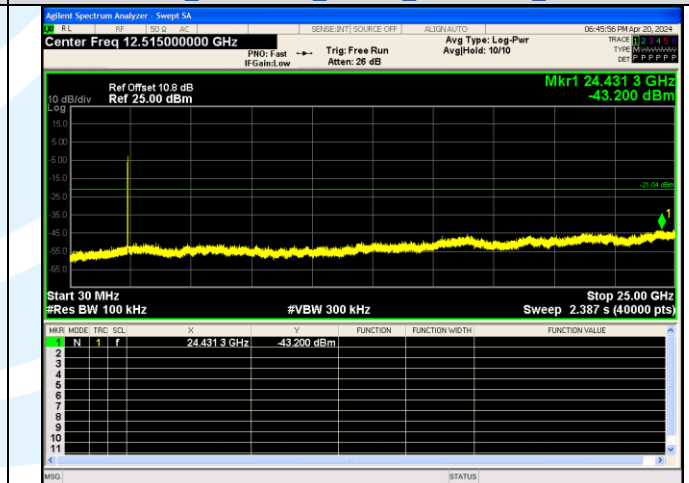
Spurious Emission IEEE 802.11ax Channel 1 20MHz Antenna 1 RU&Index SU
