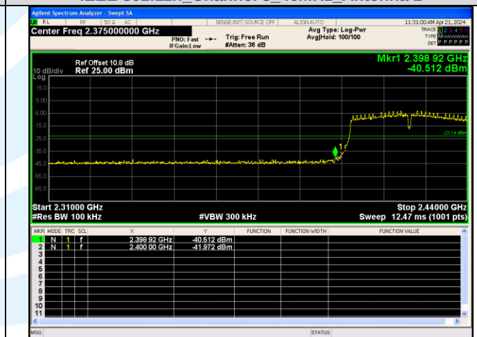
Out Of Band Emission IEEE 802.11n Channel 3 40MHz Antenna 2
