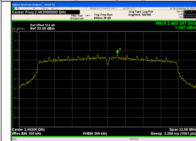
In-Band Reference Level IEEE 802.11n Channel 11 20MHz Antenna 2
