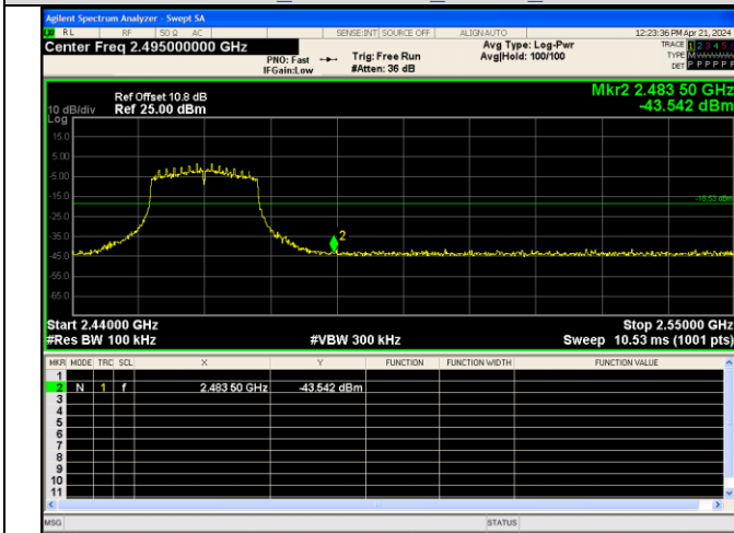
Out Of Band Emission IEEE 802.11n Channel 11 20MHz Antenna 3
