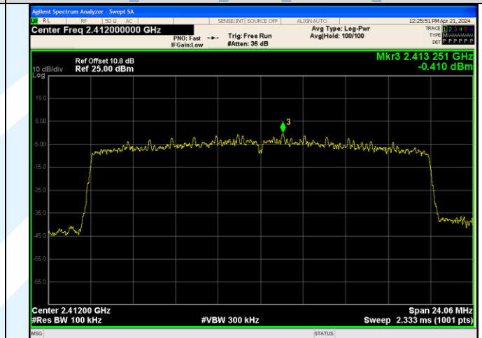
In-Band Reference Level IEEE 802.11ax Channel 1 20MHz Antenna 3 RU&Index SU
