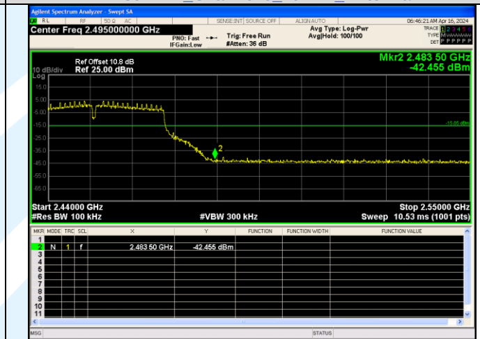
Out Of Band Emission IEEE 802.11n Channel 9 40MHz Antenna 2
