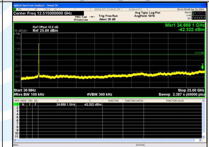
Spurious Emissions IEEE 802.11n Channel 6 40MHz Antenna 2
