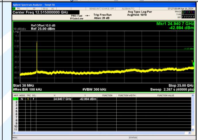
Spurious Emission IEEE 802.11g Channel 11 20MHz Antenna 3
