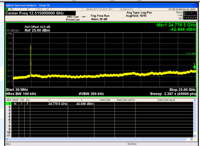
Spurious Emission IEEE 802.11n Channel 3 40MHz Antenna 3
