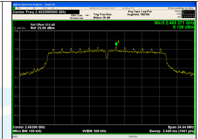
In-Band Reference Level IEEE 802.11g Channel 11 20MHz Antenna 3
