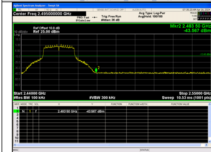
Out Of Band Emission IEEE 802.11n Channel 11 20MHz Antenna 3
