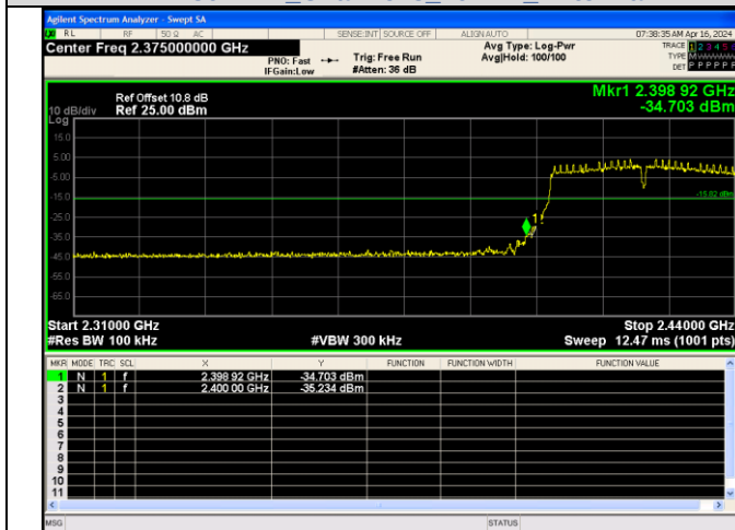
Out Of Band Emission IEEE 802.11n Channel 3 40MHz Antenna 3
