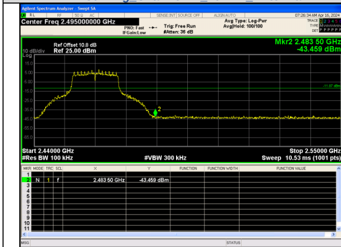
Out Of Band Emission IEEE 802.11g Channel 11 20MHz Antenna 3
