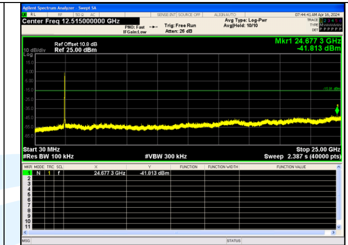
Spurious Emission IEEE 802.11n Channel 9 40MHz Antenna 3
