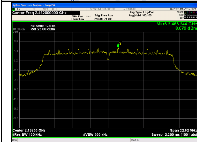
In-Band Reference Level IEEE 802.11g Channel 11 20MHz Antenna 2
