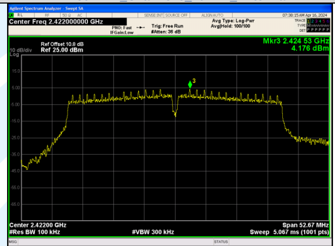
In-Band Reference Level IEEE 802.11n Channel 3 40MHz Antenna 3
