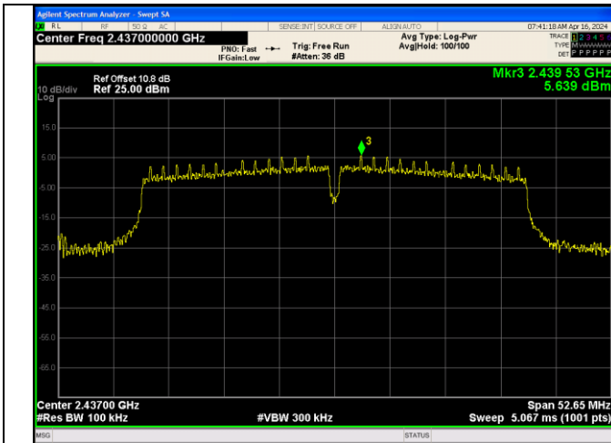
In-Band Reference Level IEEE 802.11n Channel 6 40MHz Antenna 3
