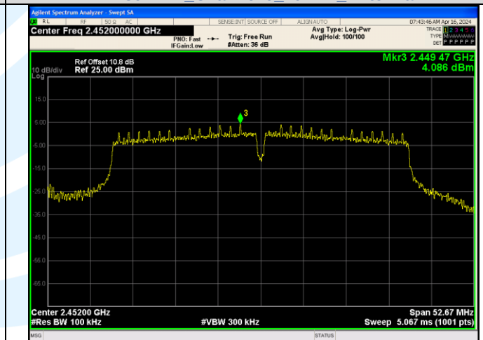
In-Band Reference Level IEEE 802.11n Channel 9 40MHz Antenna 3
