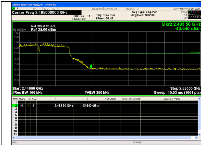
Out Of Band Emission IEEE 802.11n Channel 9 40MHz Antenna 3
