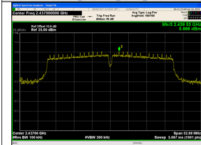
In-Band Reference Level IEEE 802.11n Channel 6 40MHz Antenna 2
