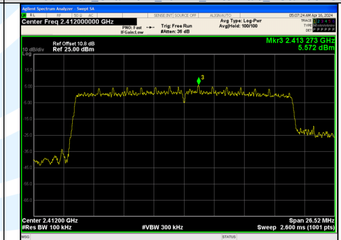
In-Band Reference Level IEEE 802.11ax Channel 1 20MHz Antenna 1 RU&Index SU
