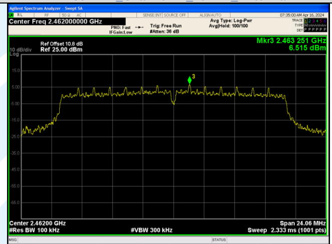
In-Band Reference Level IEEE 802.11n Channel 11 20MHz Antenna 3
