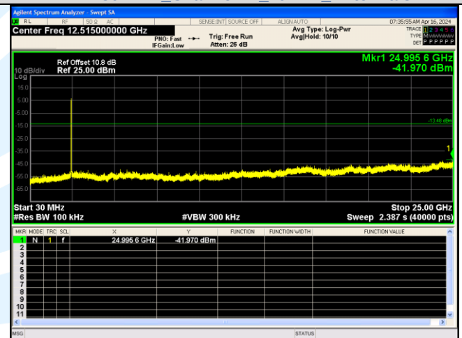
Spurious Emission IEEE 802.11n Channel 11 20MHz Antenna 3
