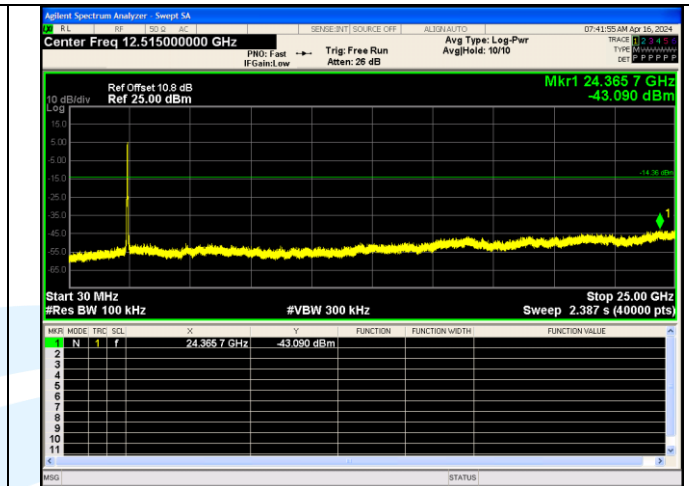
Spurious Emissions IEEE 802.11n Channel 6 40MHz Antenna 3
