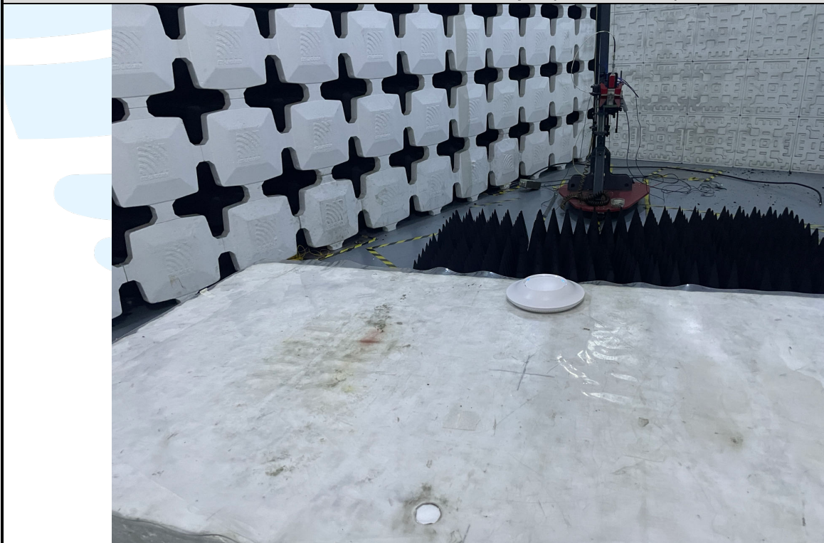
Radiated emission Test Setup-2 (Above 1 GHz)
