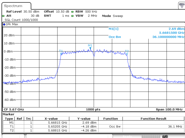
802.11ac40_5670MHz_Chain 0
