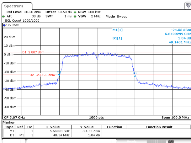
802.11ac40_5670MHz_Chain 0
