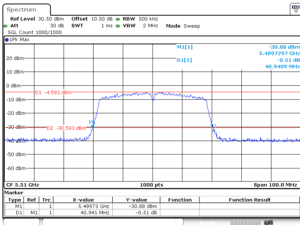
802.11ac40_5510MHz_Chain 1
