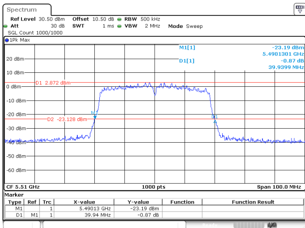
802.11ac40_5510MHz_Chain 0
