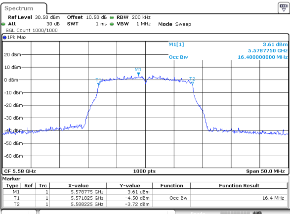
802.11a_5580MHz_Chain 0
