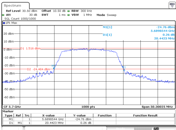
802.11a_5700MHz_Chain 1
