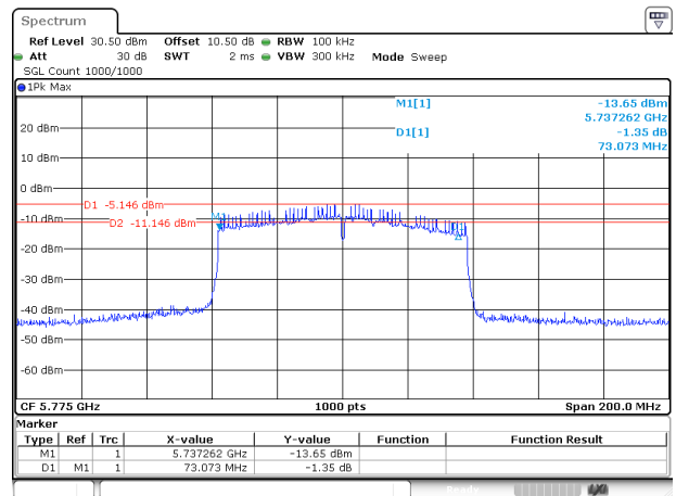
802.11ac80_5775MHz_Chain 1
