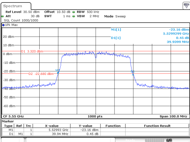
802.11ac40_5550MHz_Chain 0
