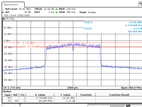
802.11ac80_5775MHz_Chain 0
