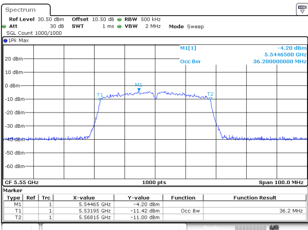
802.11ac40_5550MHz_Chain 1
