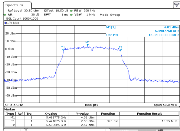
802.11a_5500MHz_Chain 0
