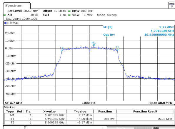
802.11a_5700MHz_Chain 0
