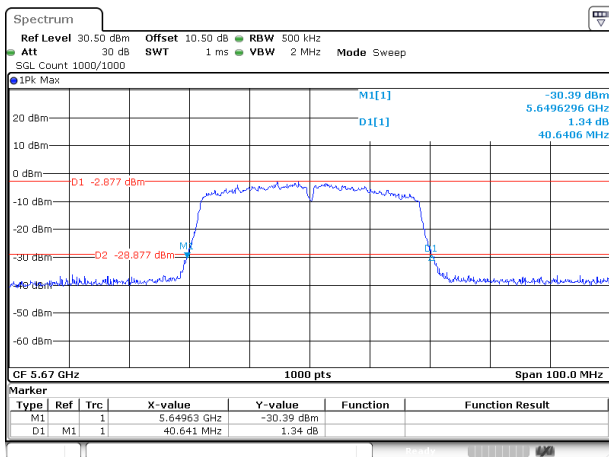
802.11ac40_5670MHz_Chain 1
