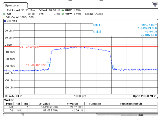
802.11ac80_5690MHz_Chain 1
