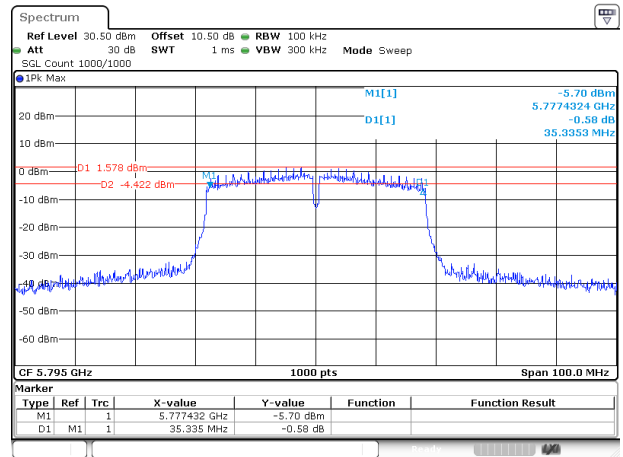
802.11ac40_5795MHz_Chain 0
