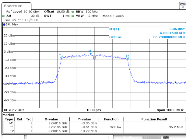
802.11ac40_5670MHz_Chain 1
