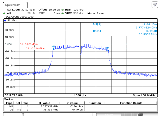
802.11ac40_5795MHz_Chain 1
