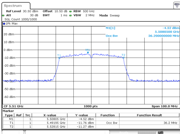
802.11ac40_5510MHz_Chain 1
