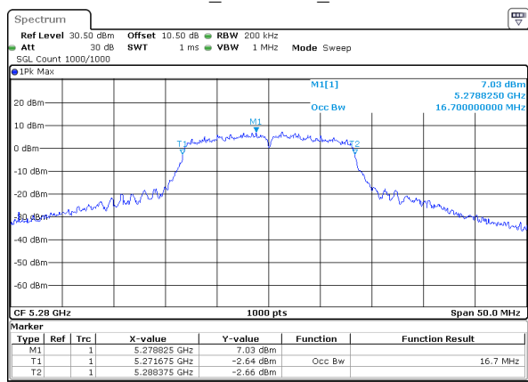
802.11a_5280MHz_Chain 1
