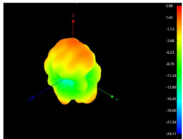
5G 3D
