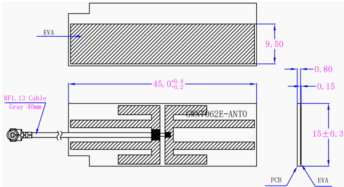
总成图 Mechanical Drawing(unit:mm)
