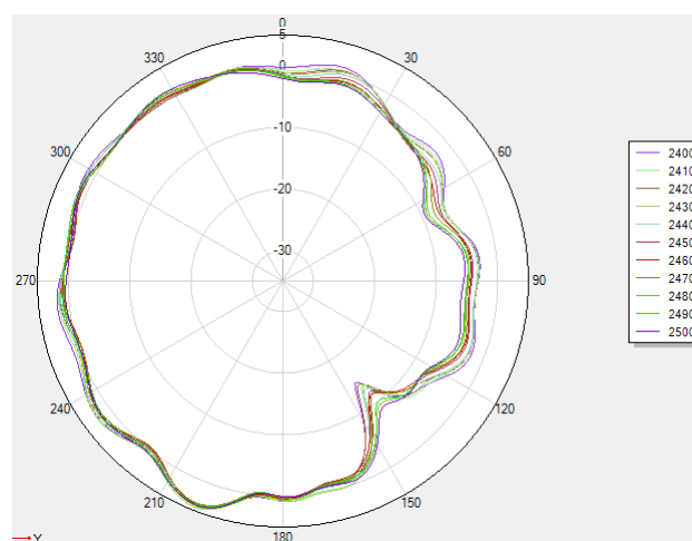
2.4G phi=90deg
