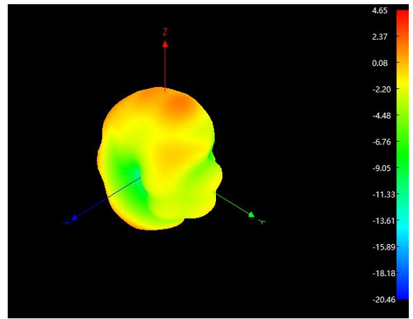
2.4G 3D
