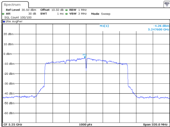
802.11ax160_5250MHz_RU_Full_Chain 0
