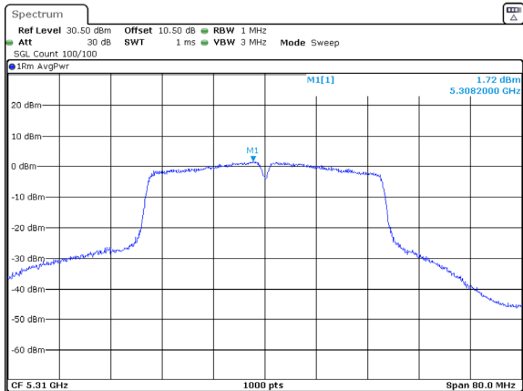
802.11ac40_5310MHz_Chain 0
