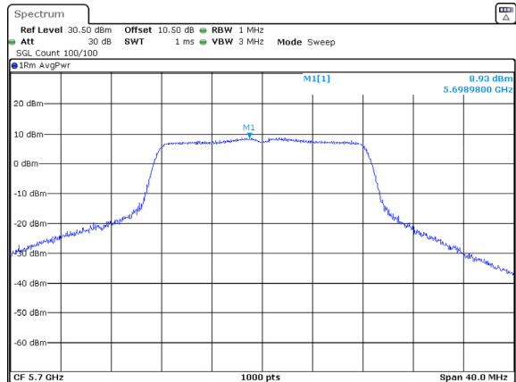
802.11a_5700MHz_Chain 2
