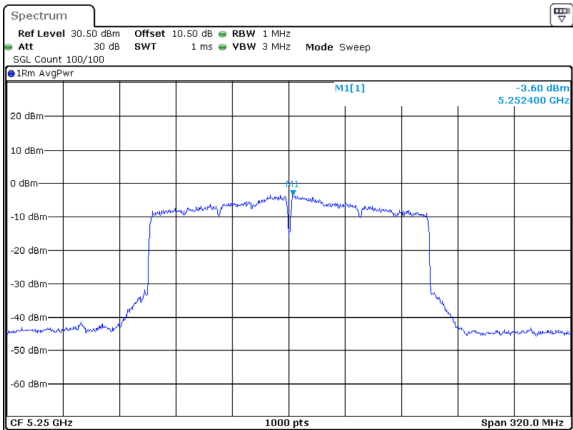
802.11ax160_5250MHz_RU_Full_Chain 1
