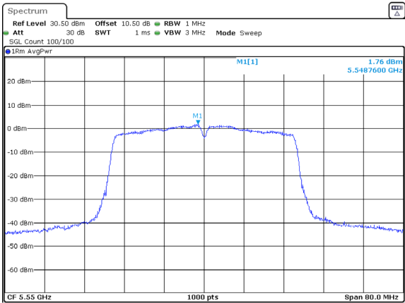
802.11ac40_5550MHz_Chain 1
