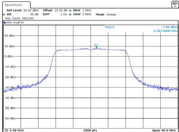
802.11a_5580MHz_Chain 2
