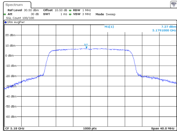
802.11ax20_5180MHz_RU_Full_Chain 0
