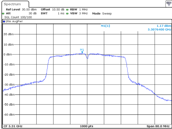
802.11ac40_5310MHz_Chain 2
