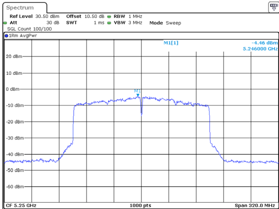
802.11ax160_5250MHz_RU_Full_Chain 2
