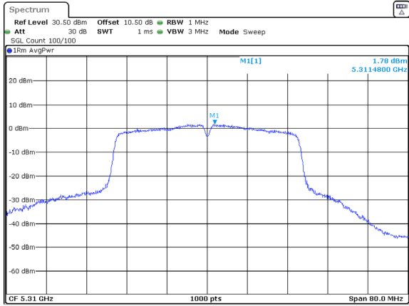
802.11ac40_5310MHz_Chain 1
