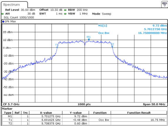
802.11a_5700MHz_Chain 2
