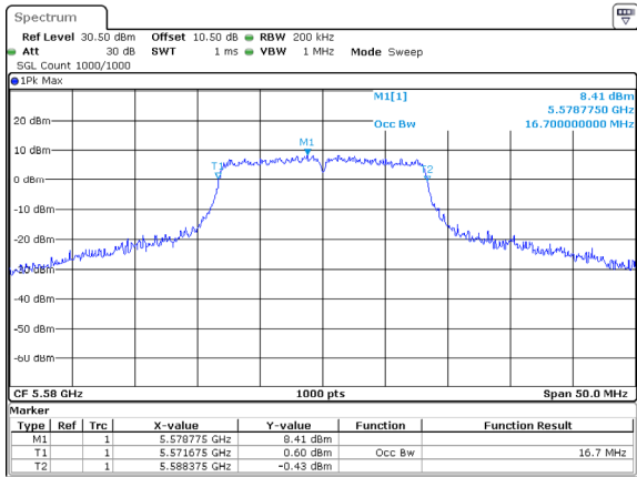
802.11a_5580MHz_Chain 2
