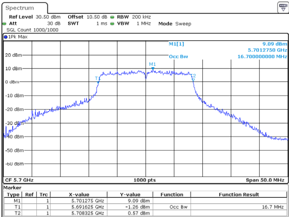
802.11a_5700MHz_Chain 1
