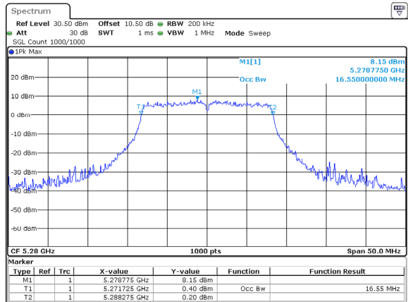
802.11a_5280MHz_Chain 2
