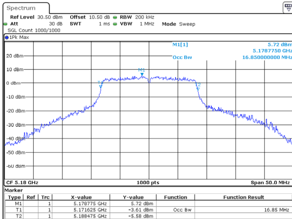
802.11a_5180MHz_Chain 2
