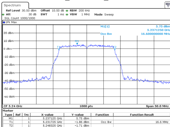
802.11a_5240MHz_Chain 2
