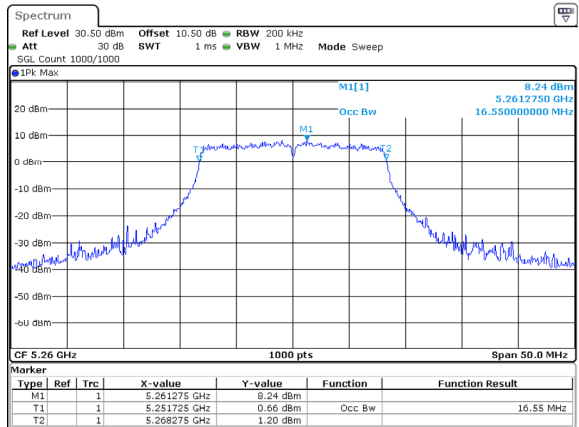
802.11a_5260MHz_Chain 2
