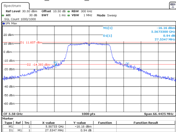
802.11a_5580MHz_Chain 1 27.535MHz
