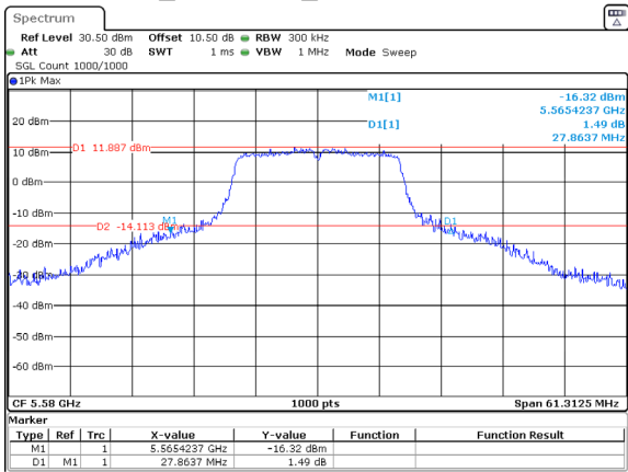
802.11a_5580MHz_Chain 0 27.864MHz
