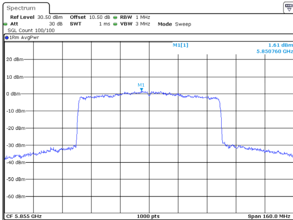
802.11ax80_5855MHz_RU_Full_Chain 1
