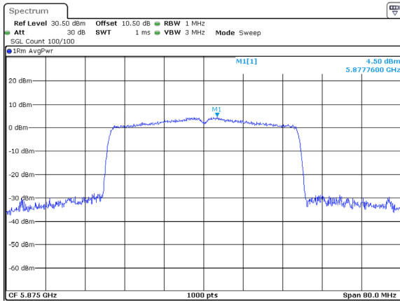
802.11ax40_5875MHz_RU_Full_Chain 2
