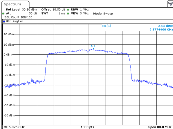
802.11ax40_5875MHz_RU_Full_Chain 1
