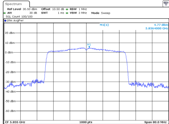
802.11ax40_5835MHz_RU_Full_Chain 2
