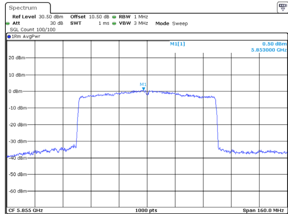
802.11ax80_5855MHz_RU_Full_Chain 2
