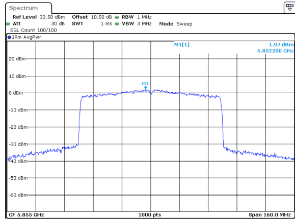
802.11ax80_5855MHz_RU_Full_Chain 0
