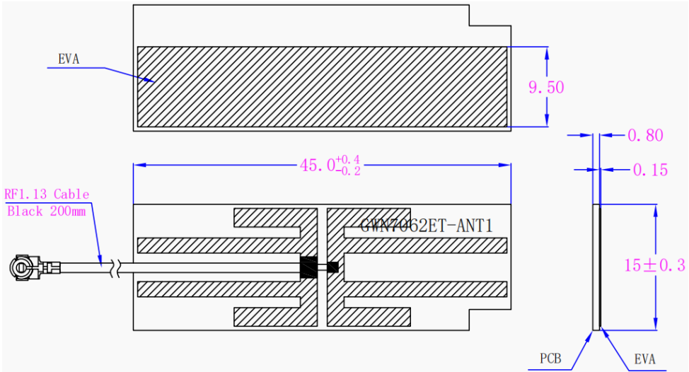
总成图 Mechanical Drawing(unit:mm)
