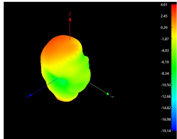
2.4G 3D
