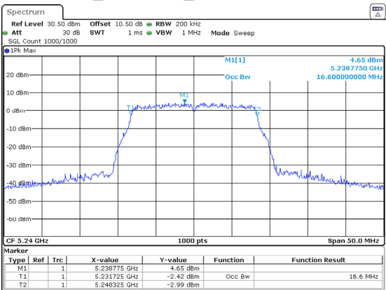
802.11a_5240MHz_Chain 2 16.600MHz
