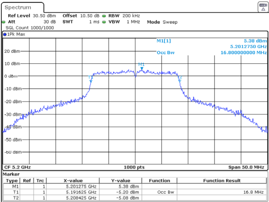
802.11a_5200MHz_Chain 2 16.800MHz
