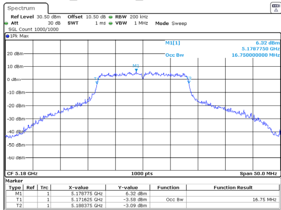
802.11a_5180MHz_Chain 0 16.750MHz
