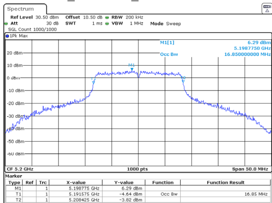
802.11a_5200MHz_Chain 1 16.850MHz
