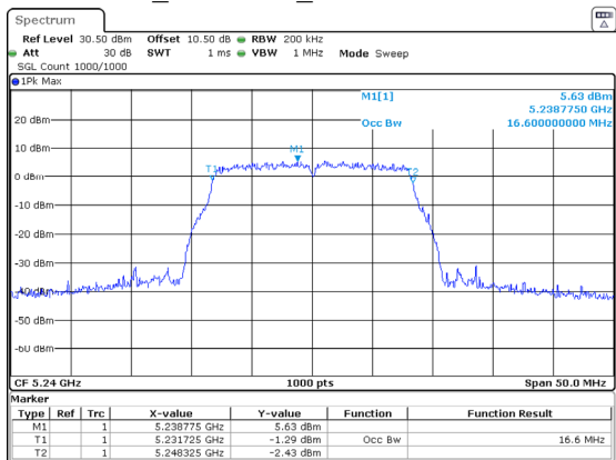
802.11a_5240MHz_Chain 1 16.600MHz
