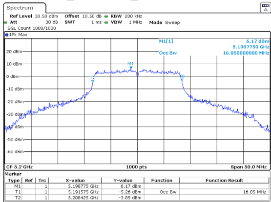
802.11a_5200MHz_Chain 0 16.850MHz
