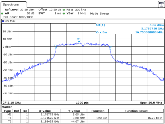
802.11a_5180MHz_Chain 2 16.750MHz
