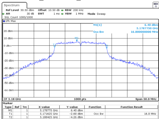
802.11a_5180MHz_Chain 1 16.800MHz
