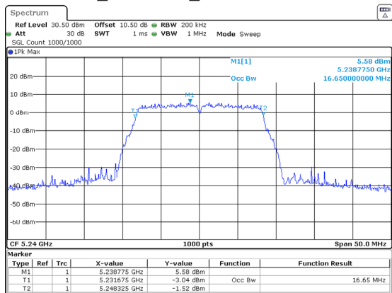
802.11a_5240MHz_Chain 0 16.650MHz
