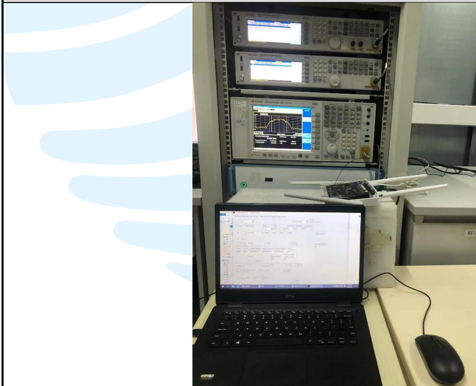
RF Conducted Test Setup
