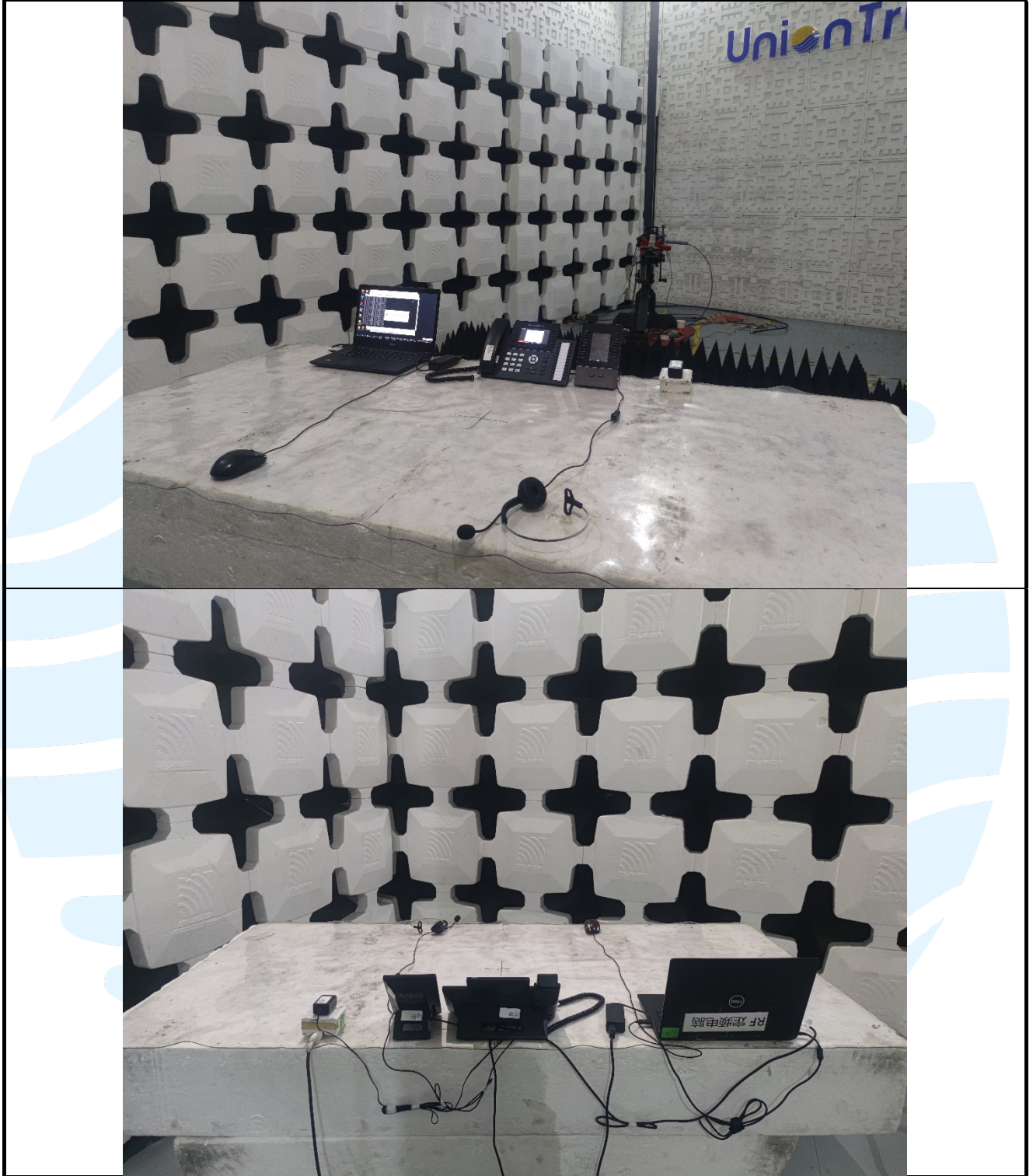
Radiated emission (AC Port) Test Setup-2 (Above 1 GHz)
