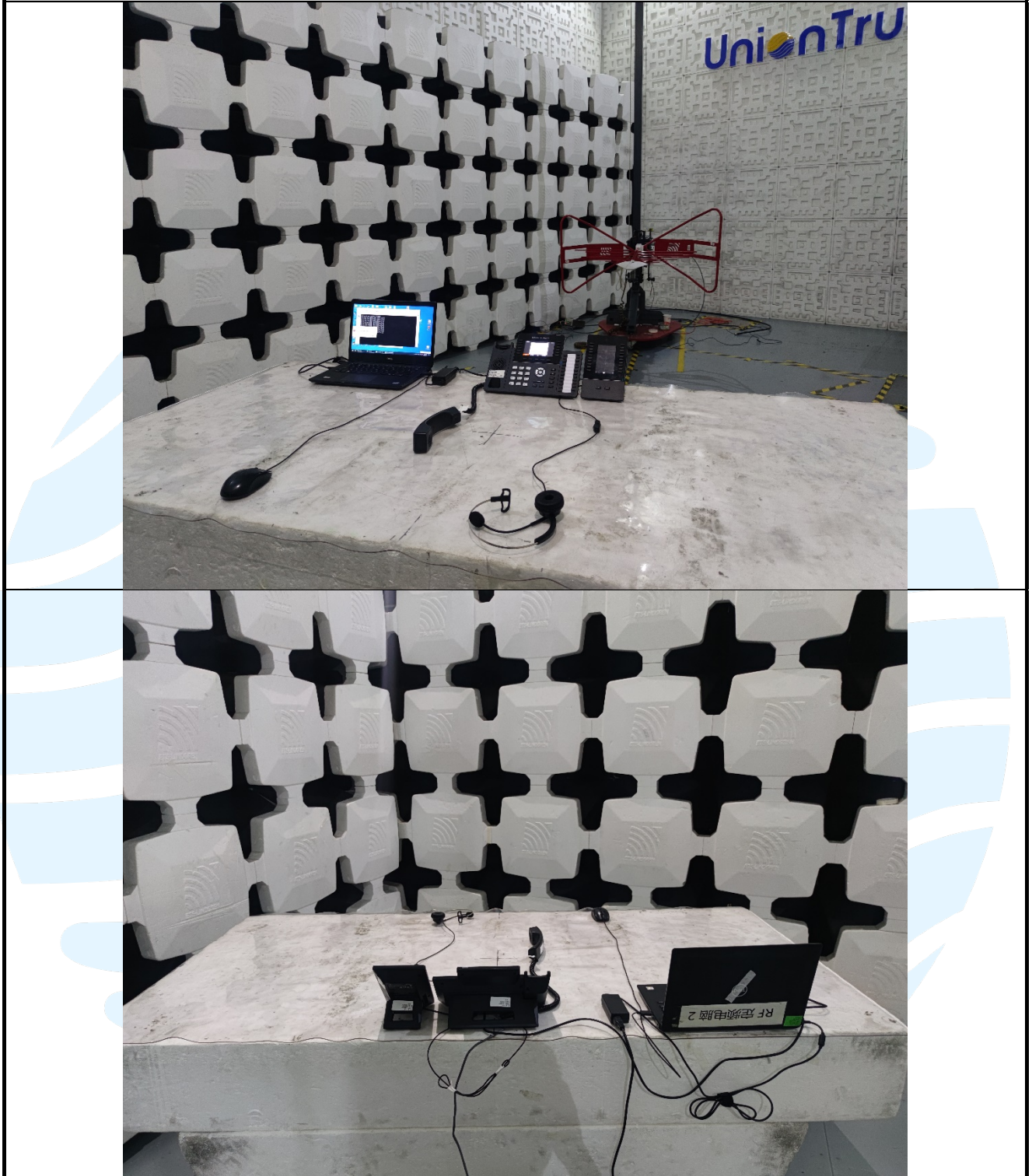
Radiated emission (PoE Port) Test Setup-3 (30 MHz~1 GHz)
