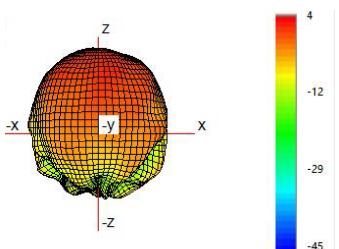
5G 3D
