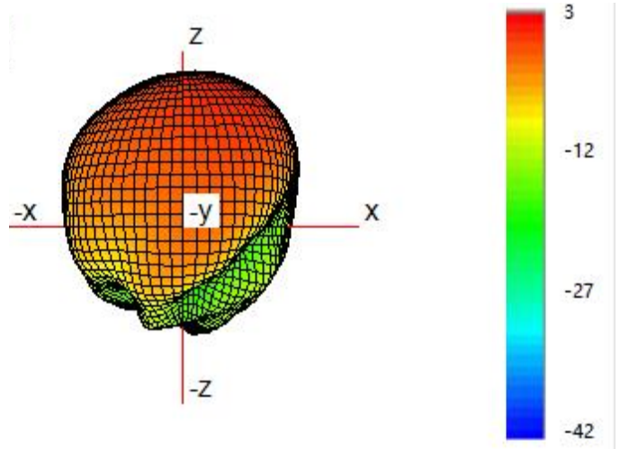
2.4G 3D
