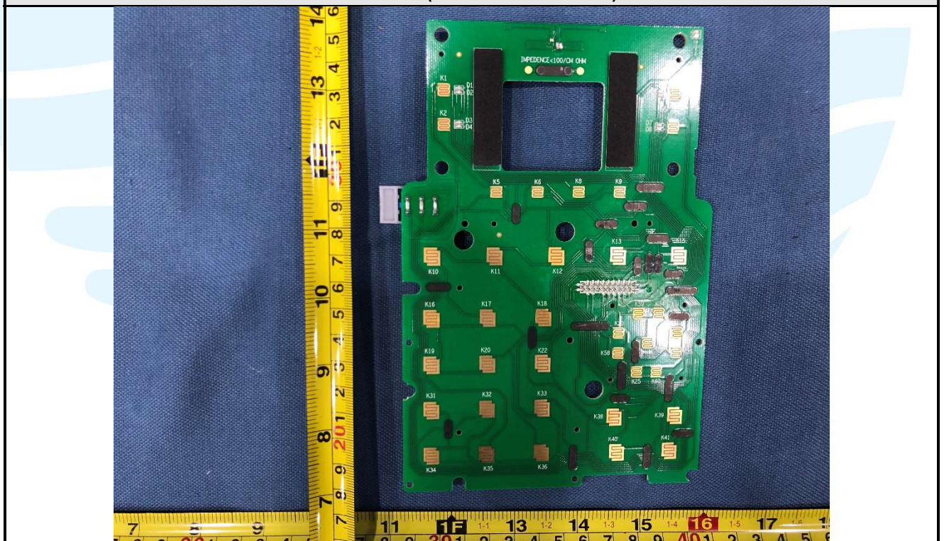
EUT Photo (Model No.:GRP2612)
