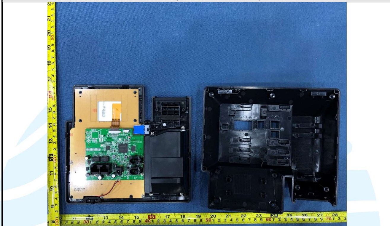
EUT Photo (Model No.:GRP2612P)
