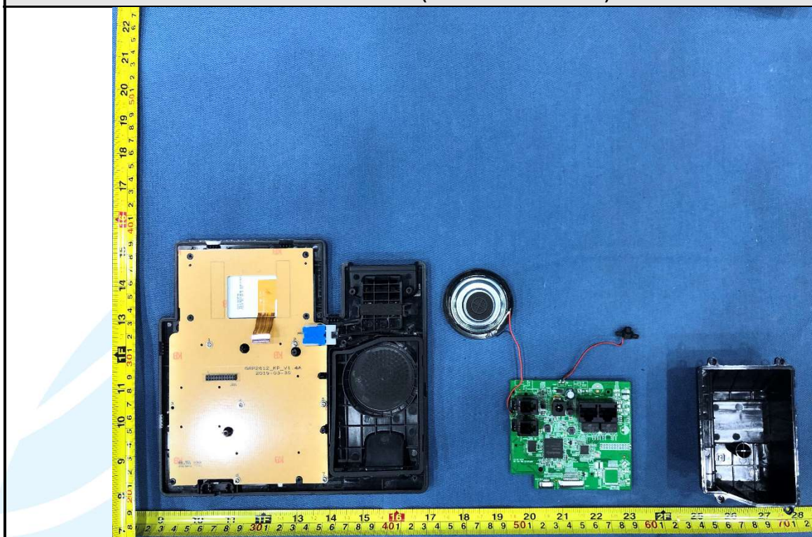
EUT Photo (Model No.:GRP2612)
