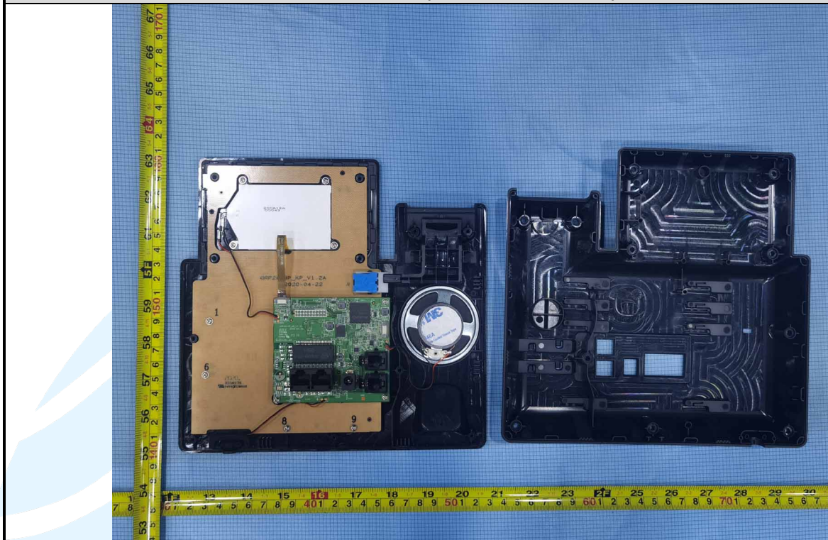
EUT Photo (Model No.:GRP2603)
