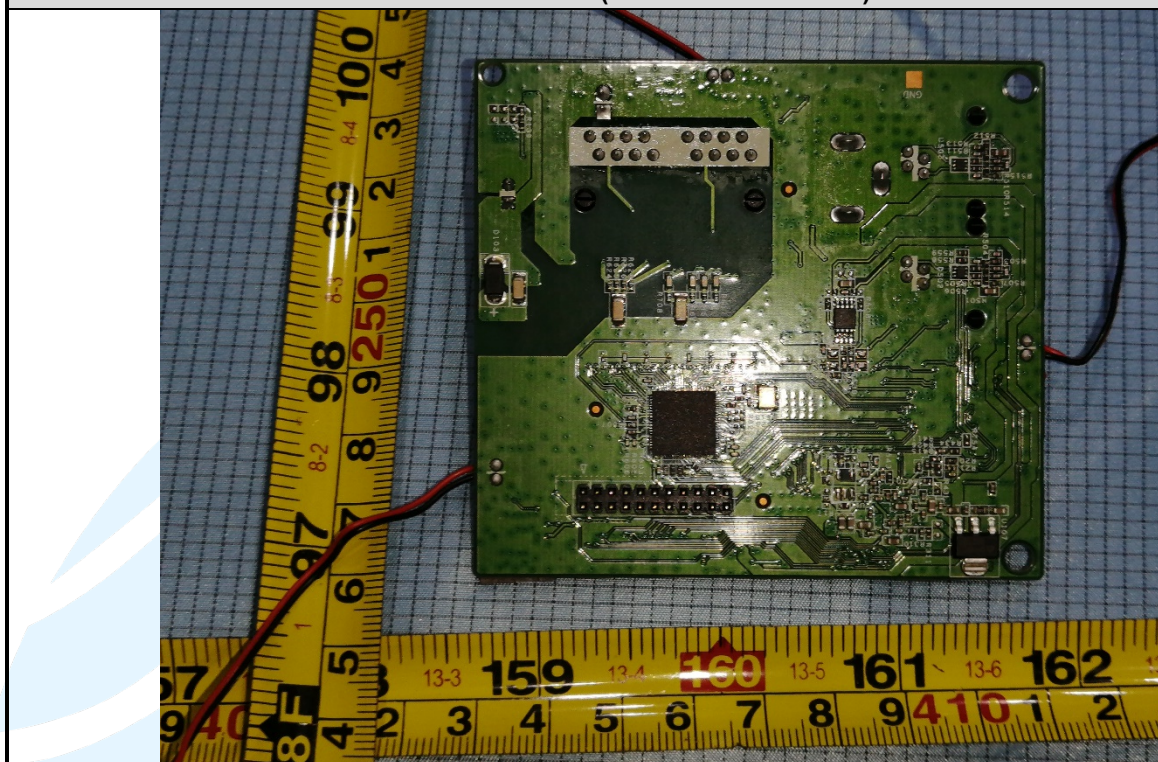
EUT Photo (Model No.:GRP2603)
