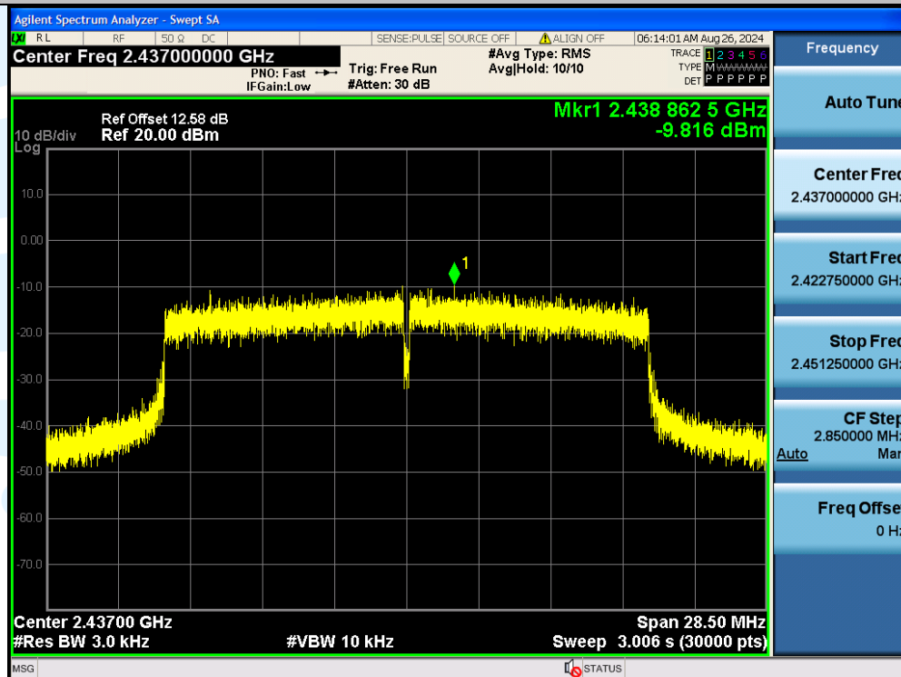
11AX20SISO-Ant1-2437-PASS
