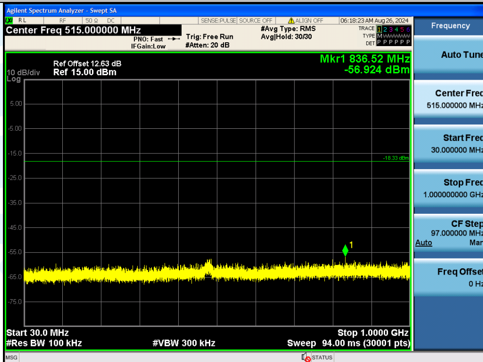
11AX20SISO-Ant1-2462-30~1000-PASS
