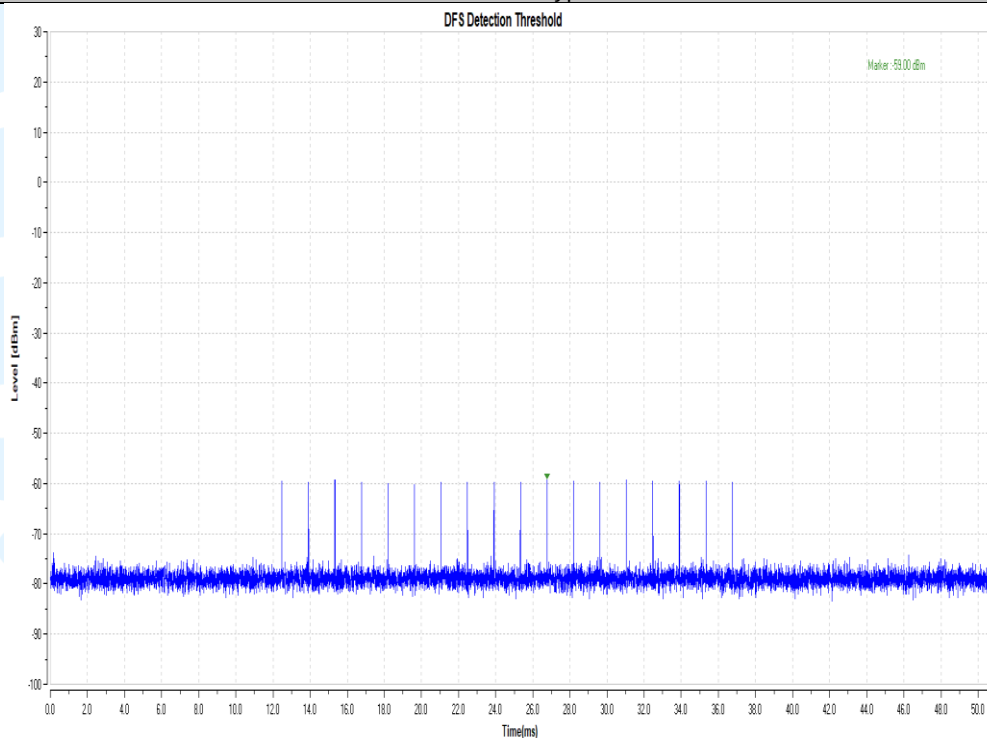
11AX40SISO-5310-Type0-PASS
