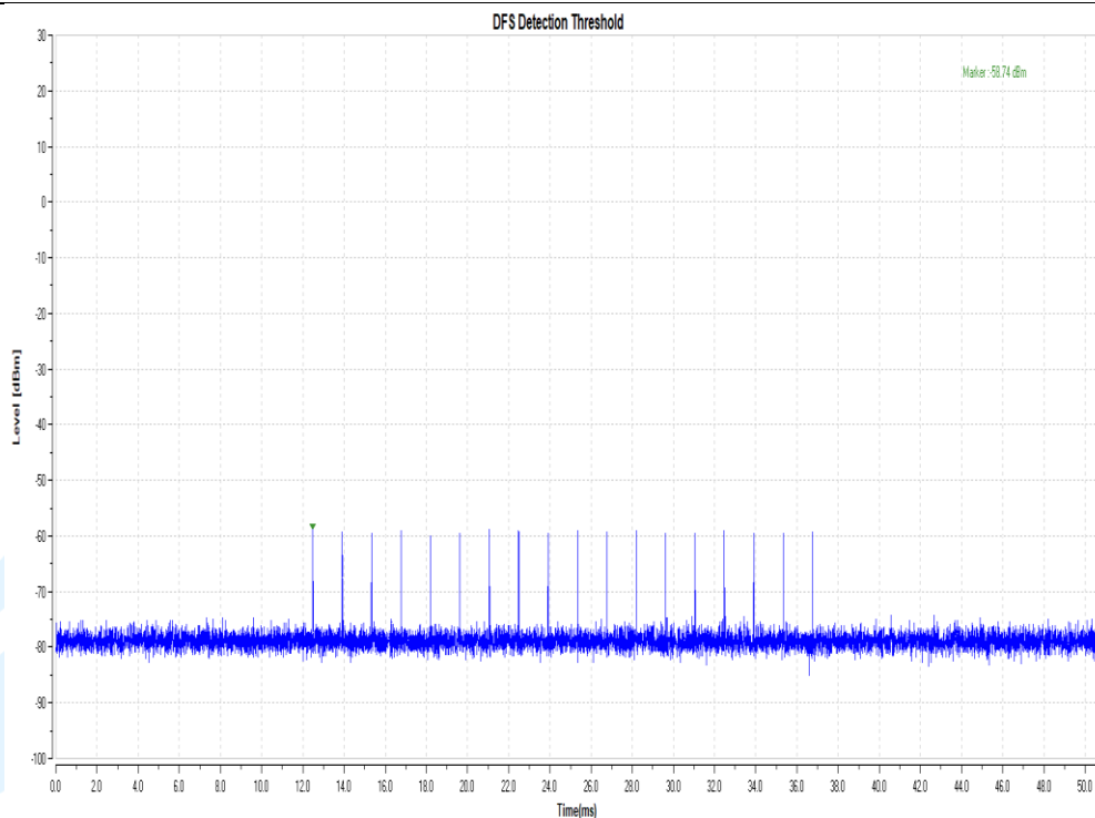
11AX20SISO-5500-Type0-PASS
