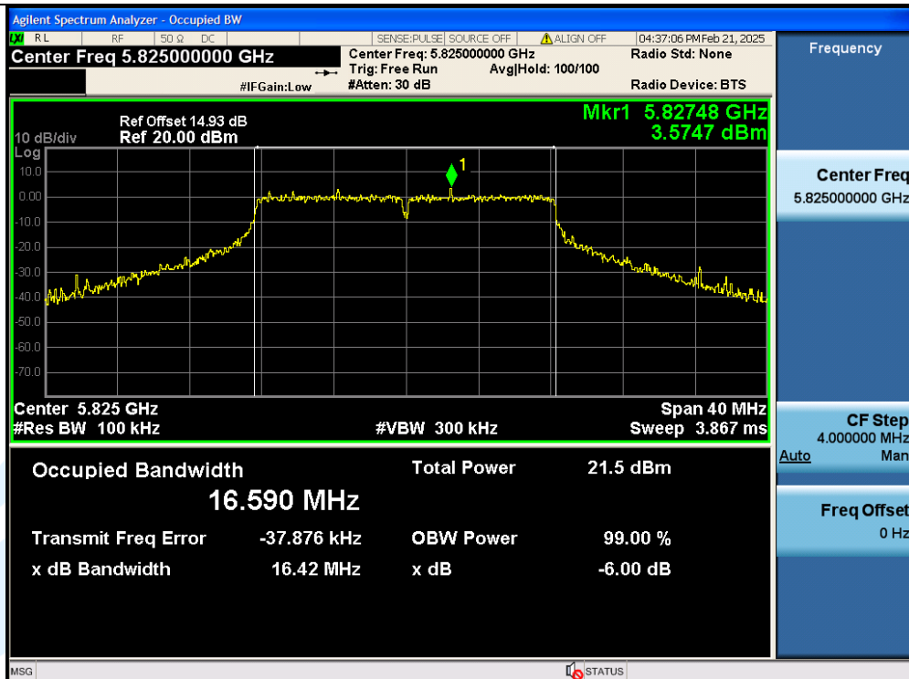
11A-Ant1-5825-PASS
