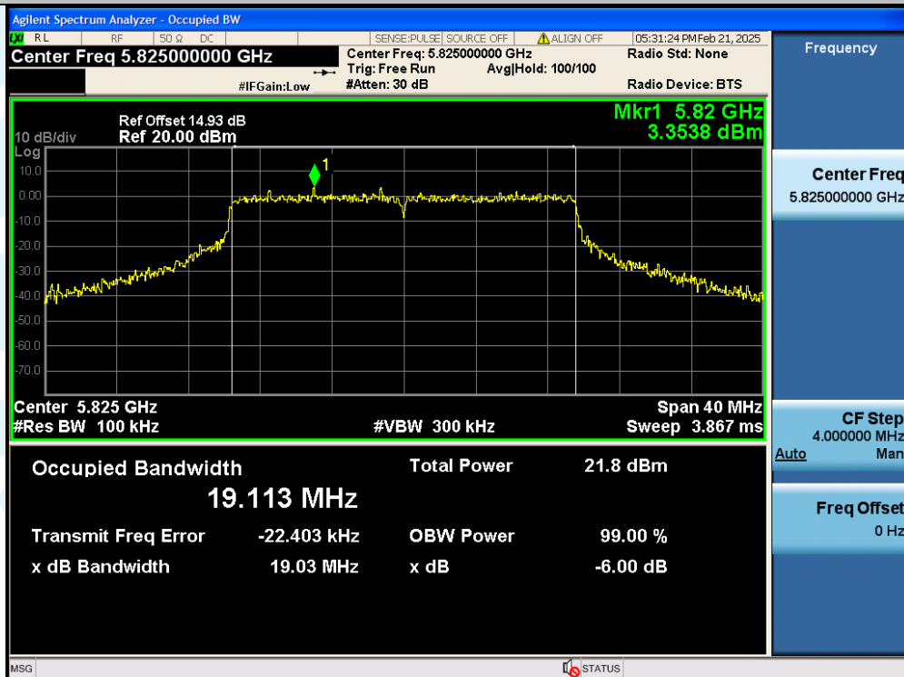
11AX20SISO-Ant1-5825-PASS
