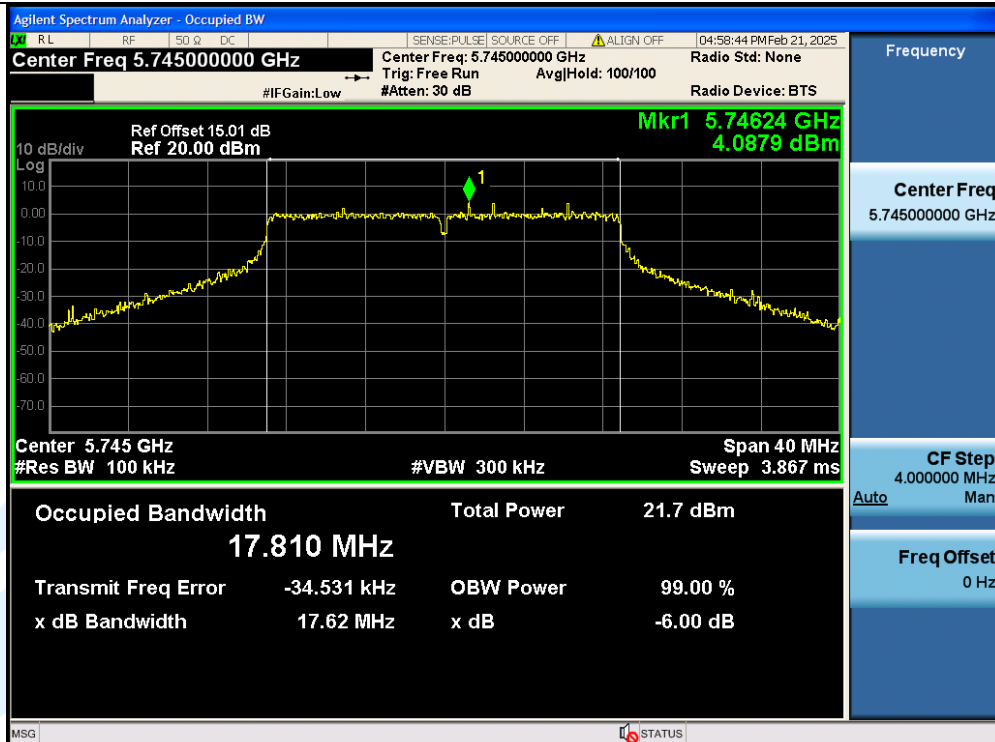
11AC20SISO-Ant1-5745-PASS
