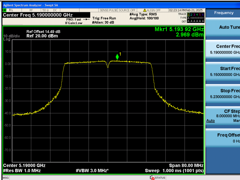
11N40SISO-Ant1-5190-PASS
