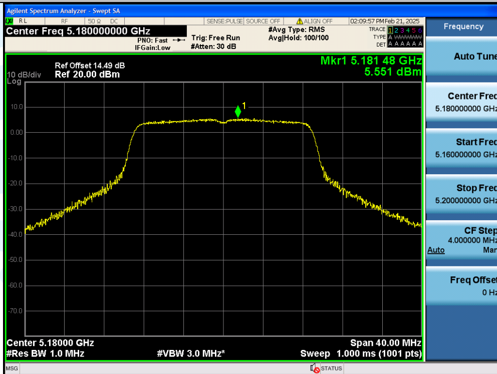
11N20ISO-Ant1-5180-PASS
