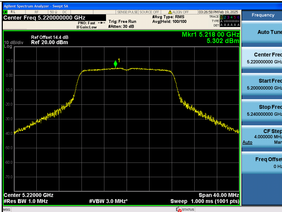
11A-Ant1-5220-PASS
