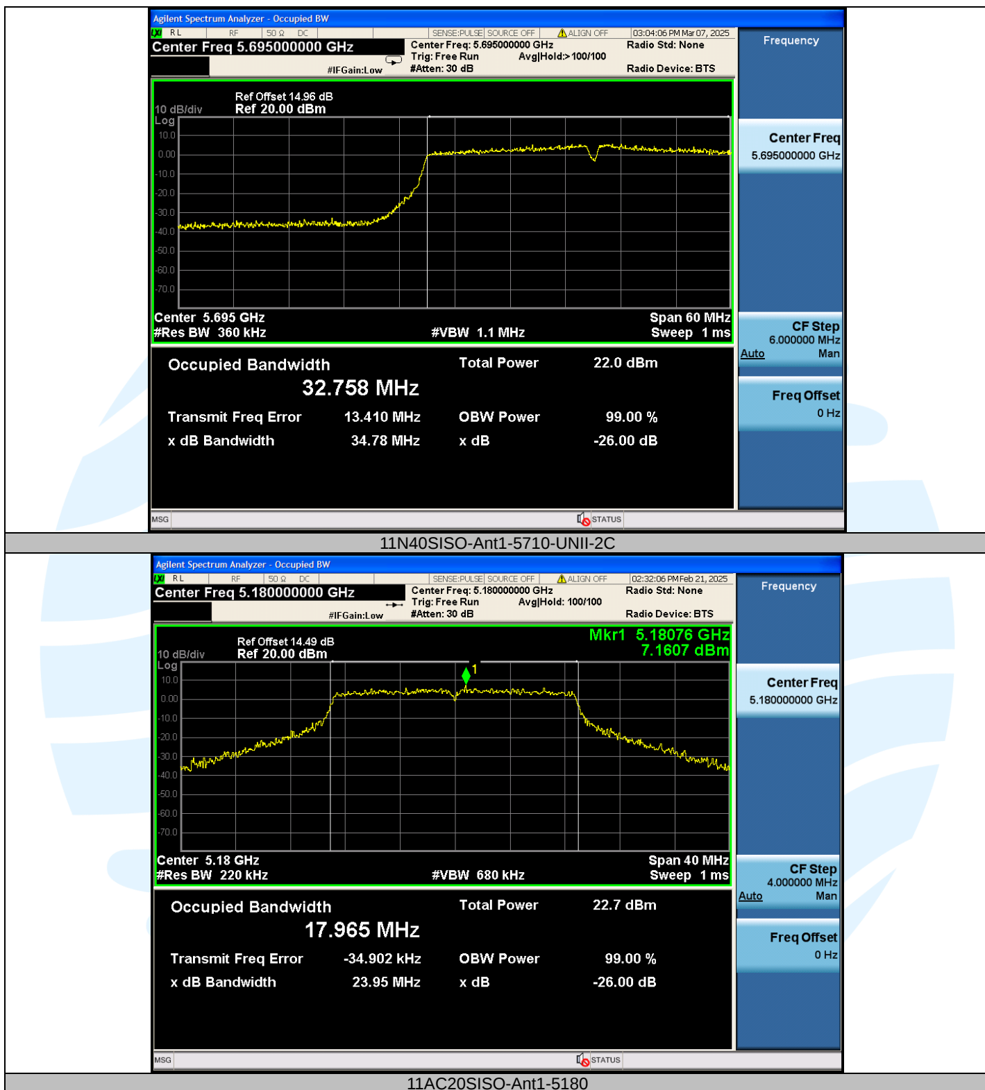
11AC20SISO-Ant1-5180
