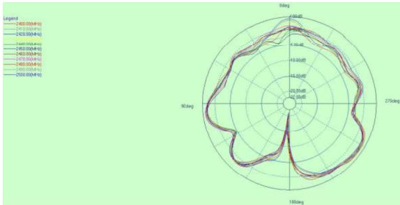
2.4G phi=90deg
