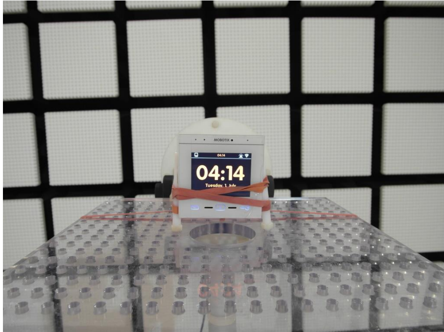
Photo 1 (RSE set-up / Fully-anechoic chamber):
