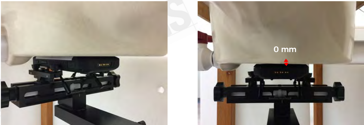
Fig.16 EUT Front side to flat phantom
