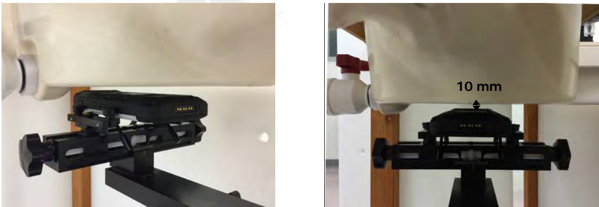
Fig.11 EUT Back side to flat phantom
