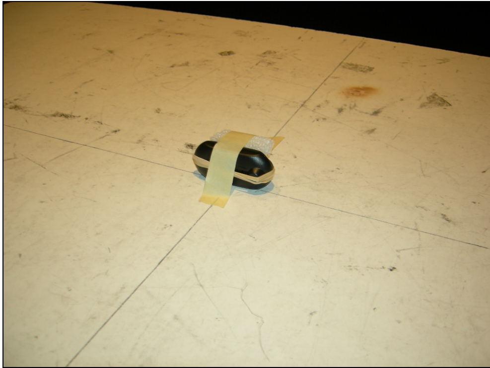
Figure 5: Radiated Emissions Test Setup – Z-POS – Front View
