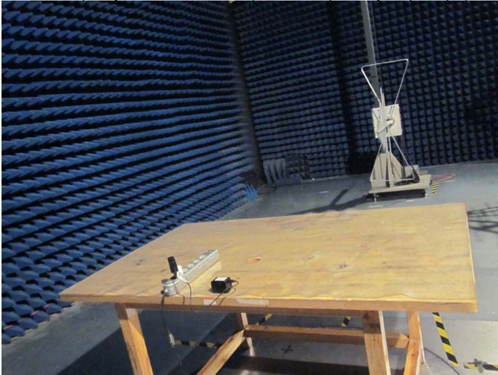
Test frequency from 30MHz to 1GHz( Wifi mode , power by adapter input)
