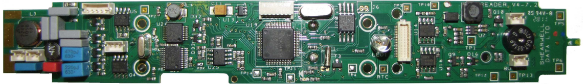
SDL400S top of Board with Bluetooth module and display boards removed
