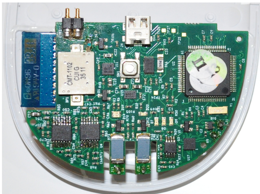
Aingeal Device View of PCB underside
