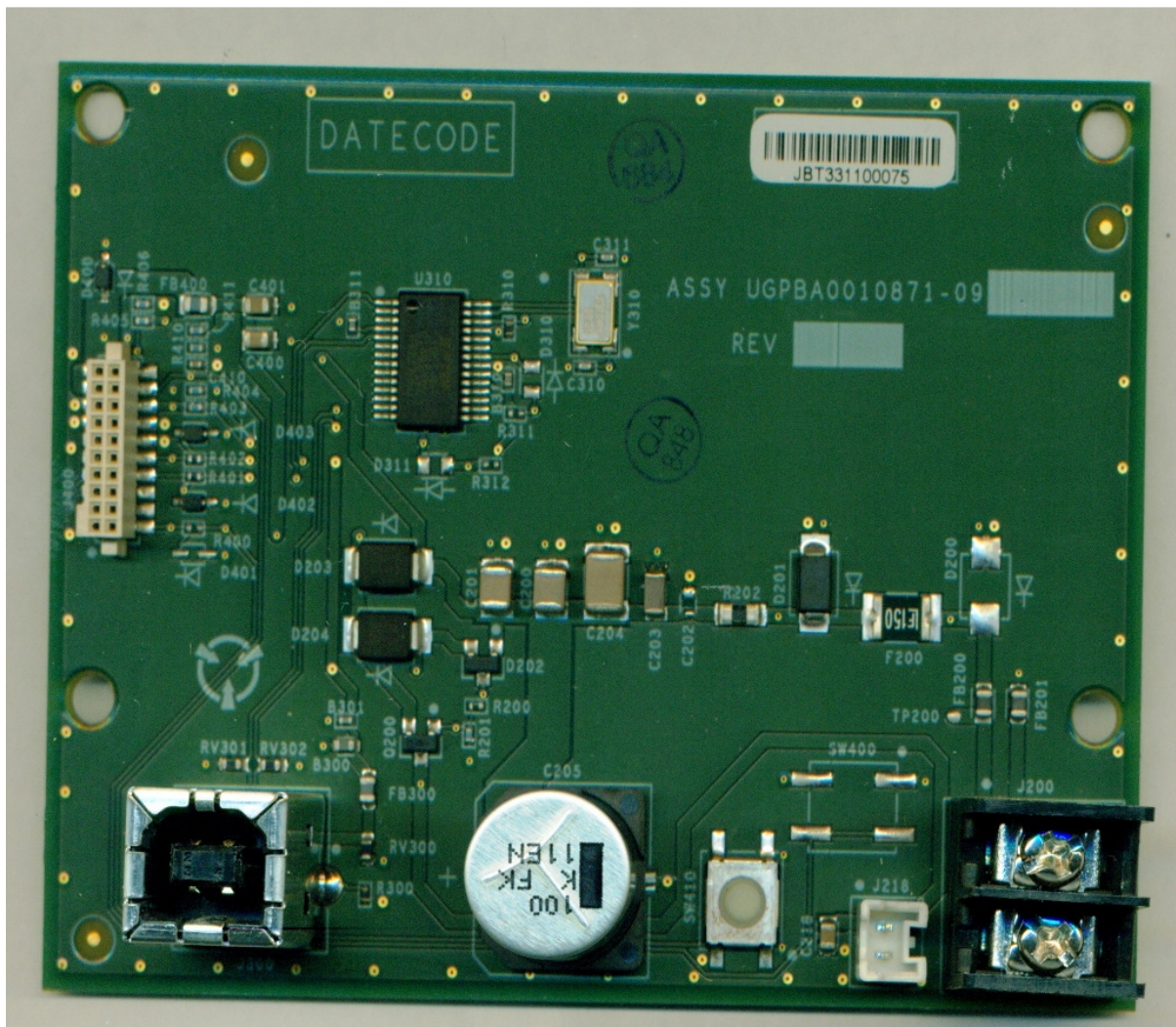
Photo 3 – Top View of the Main Board
