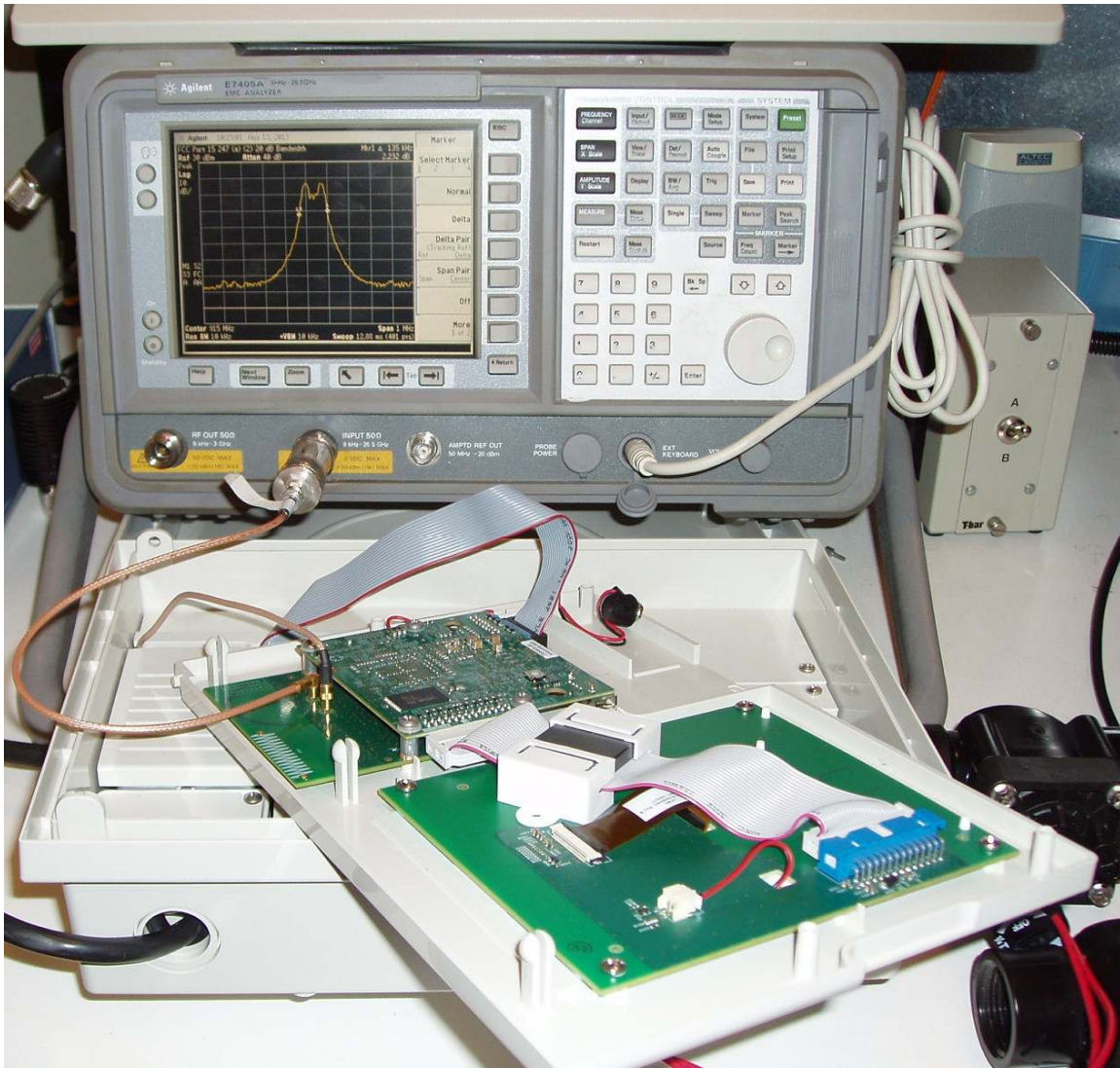
Photo 5 – Antenna Port Conducted Test Set-up
