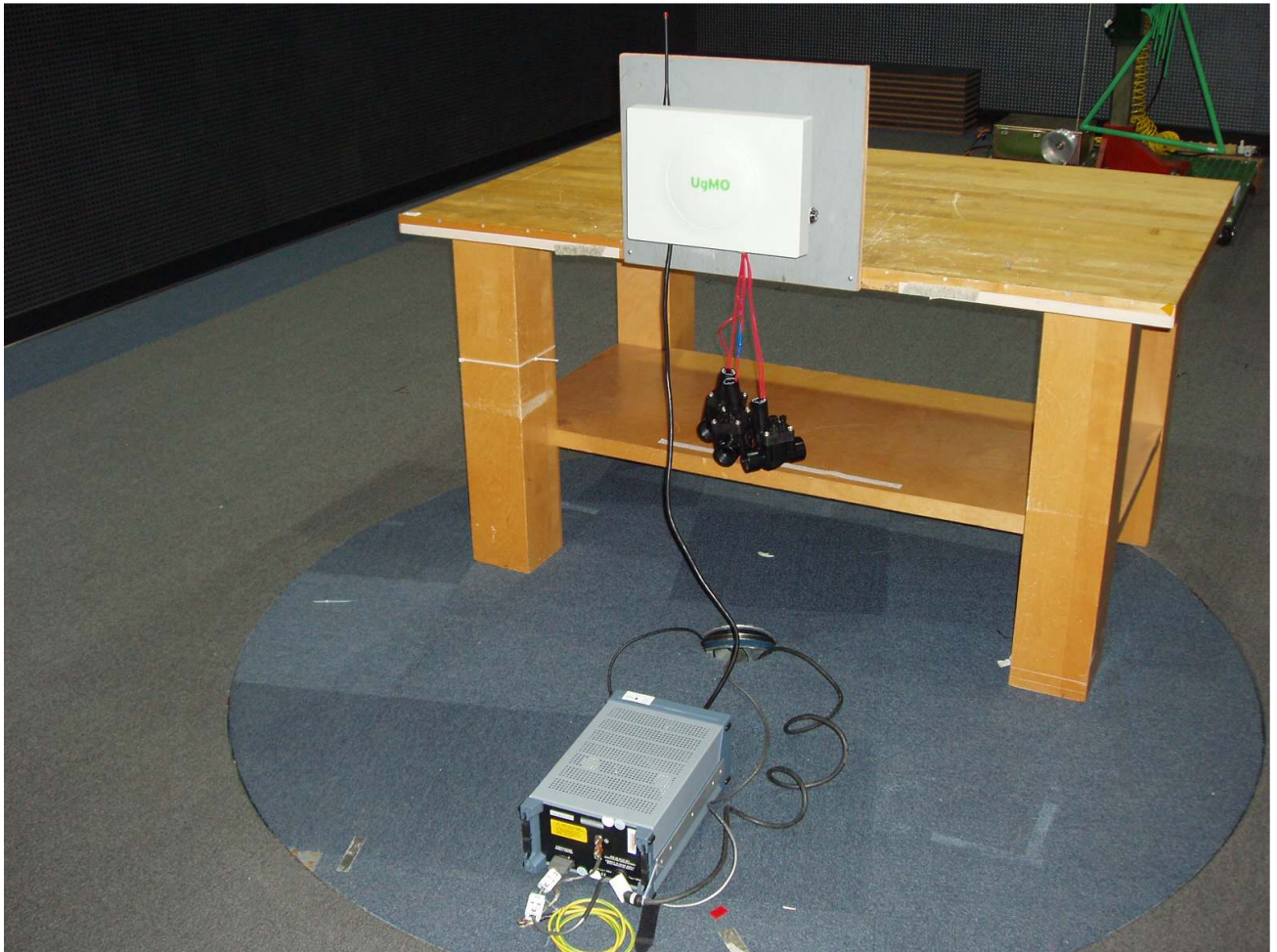
Photo 6 – AC Mains Conducted Emissions Test Set-up
