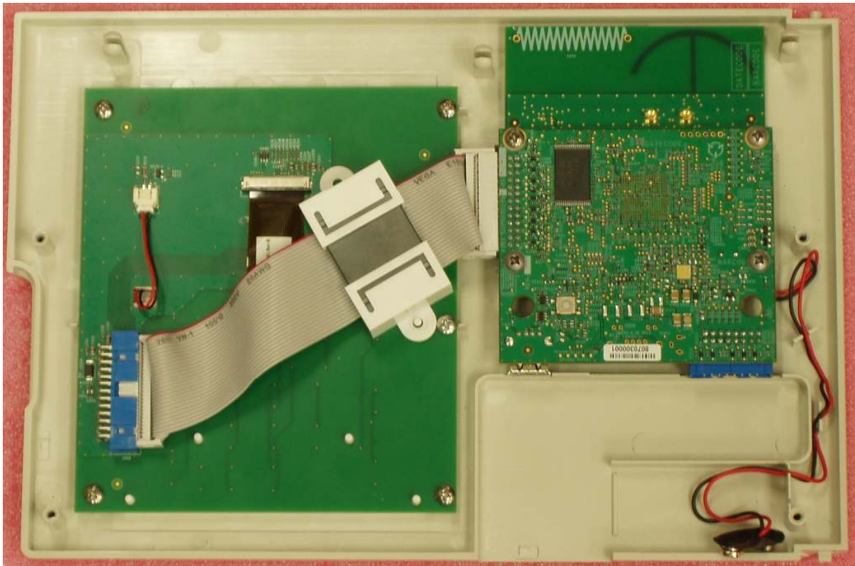
Photo 5 – Boards Mounted in the Front Panel Subassembly
