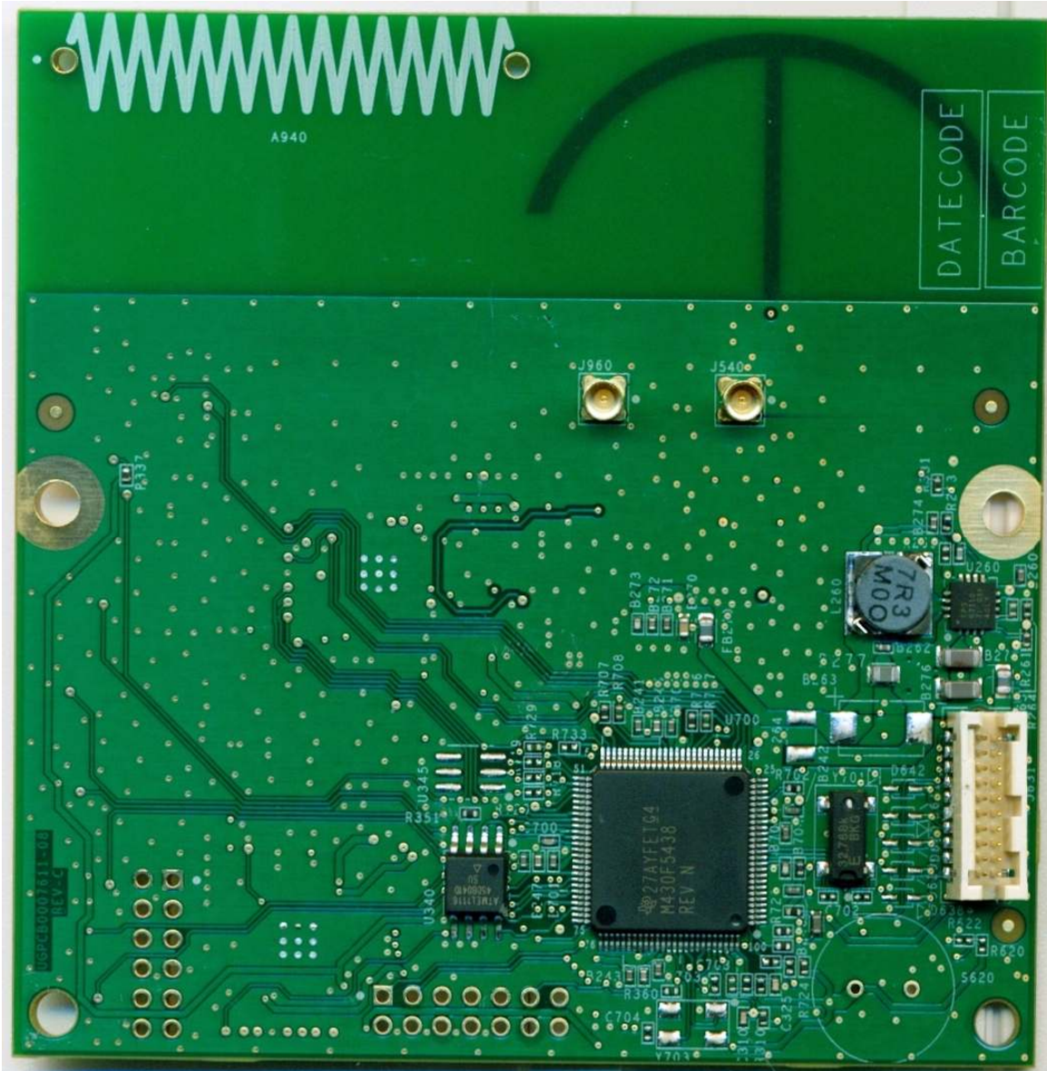
Photo 1 – Top View of the Radio Board
