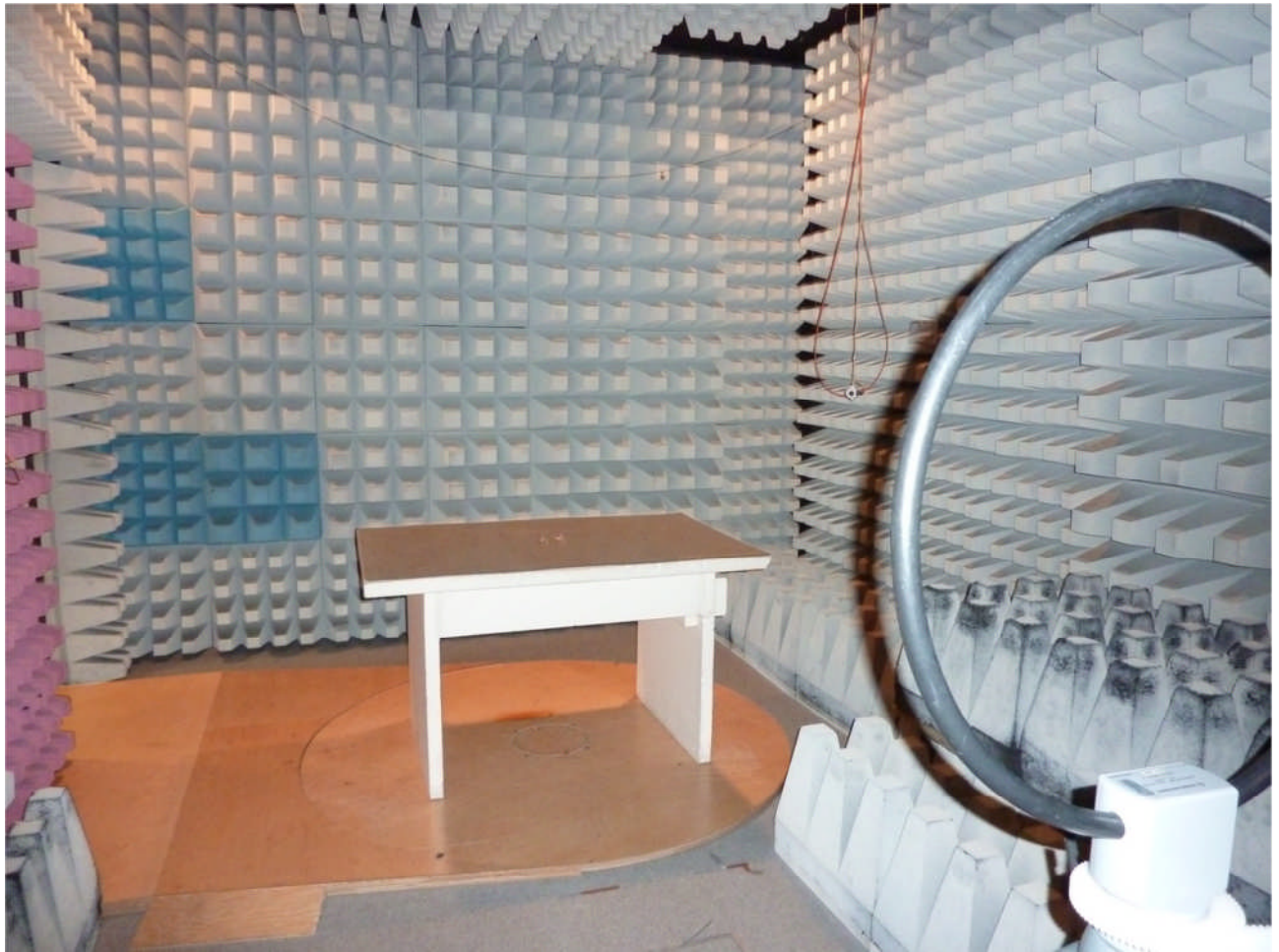
113677emi4.JPG: Test set-up radiated emission (H-Field)
