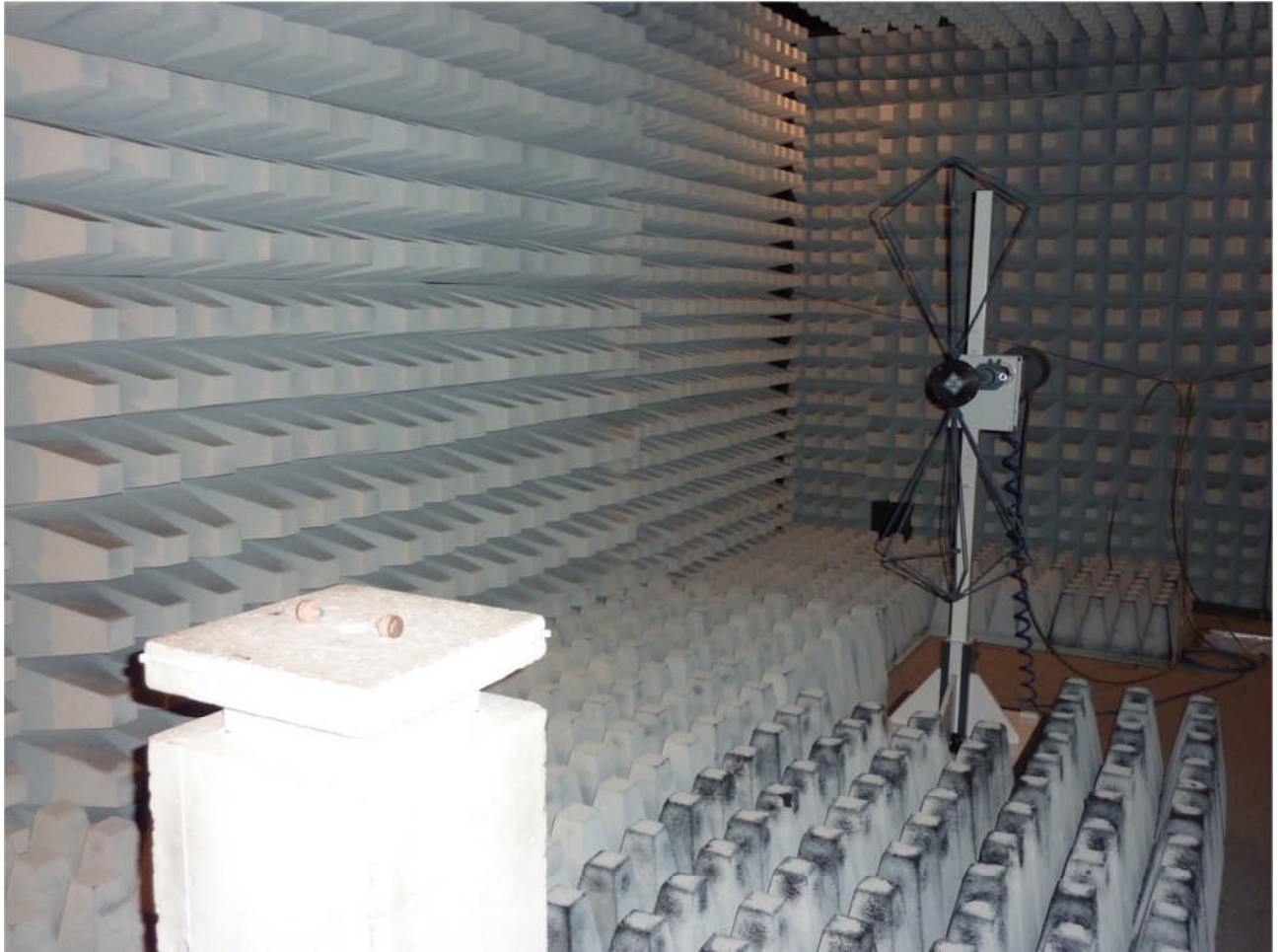
113677emi3.JPG: Test set-up radiated emission (E-Field)
