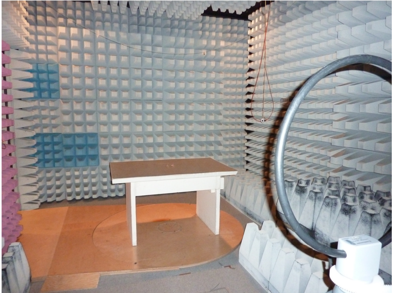
120962emi2.JPG: Test set-up preliminary radiated emission (H-Field)
