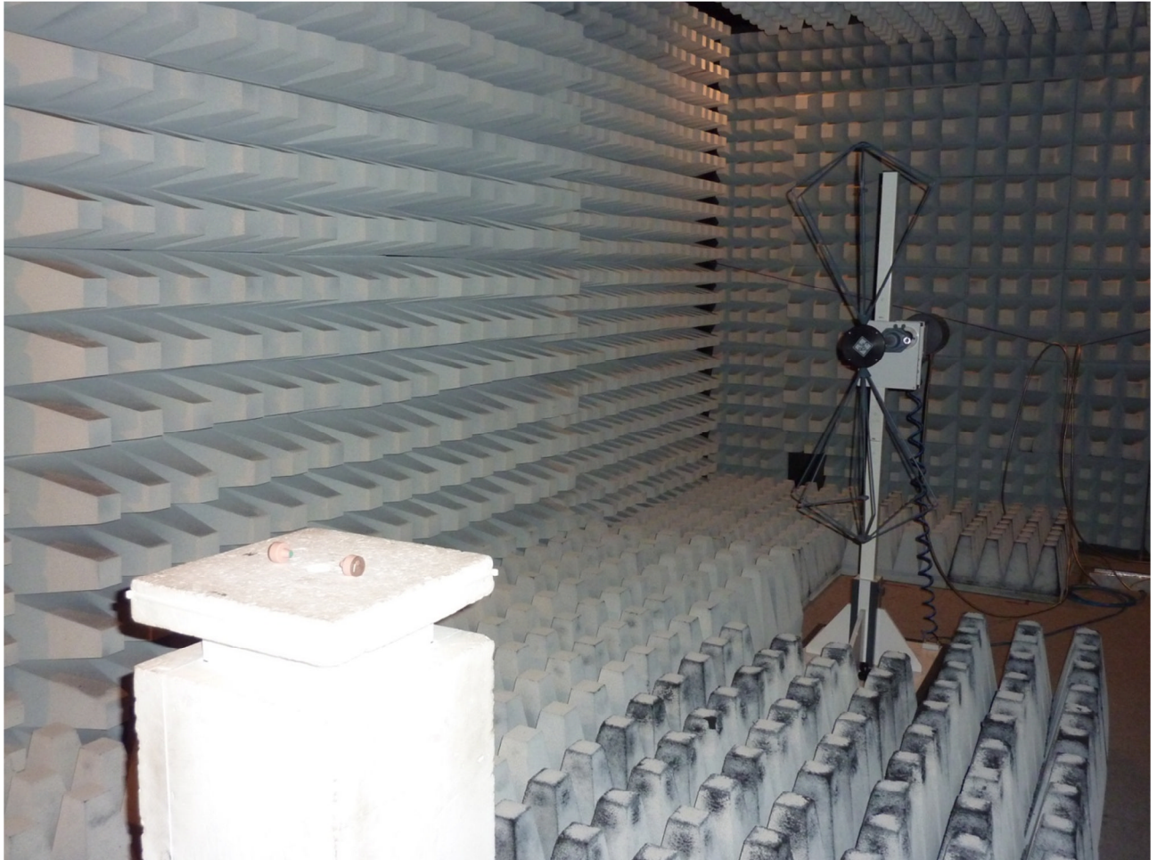
120962emi1.JPG: Test set-up radiated emission (E-Field)
