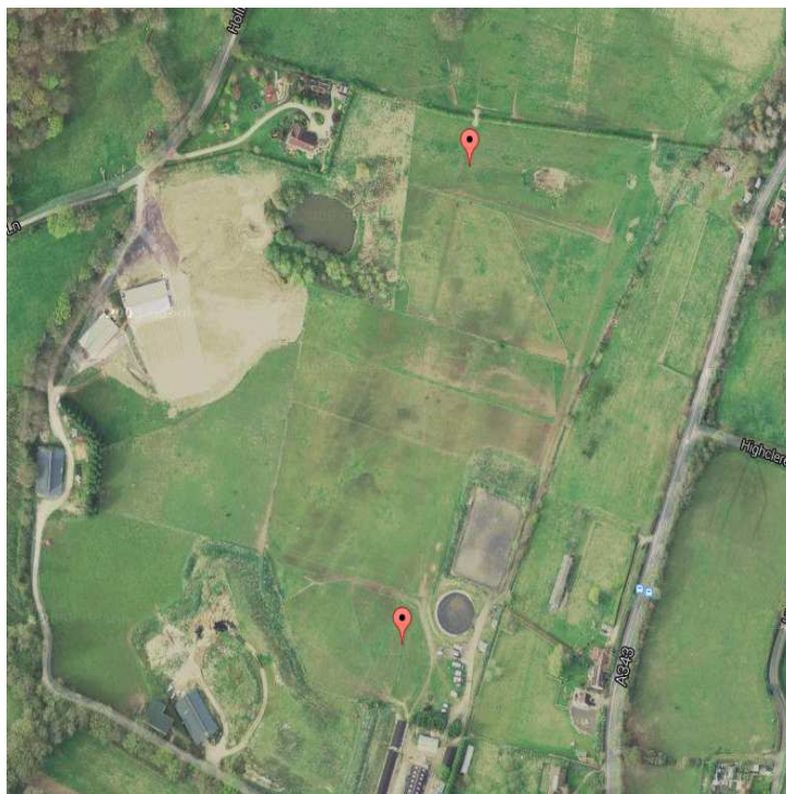
Aerial view of test site. Red markers indicates test locations. EUT located at upper marker. Mag loop antenna located at lower marker.
