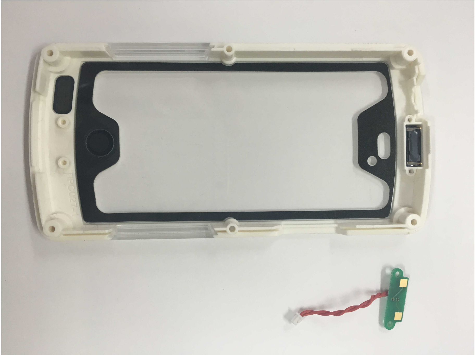
InfineaX - upper enclosure back view and front speaker PCB C018501
