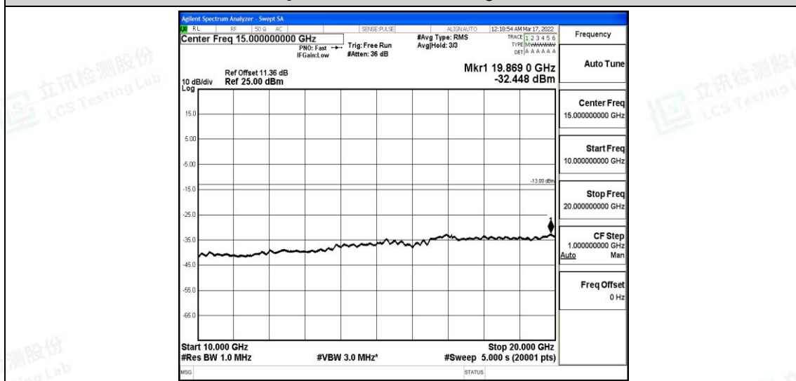
Band2-20MHz-16QAM-19100-1RB#0-Range5:10000~20000MHz
