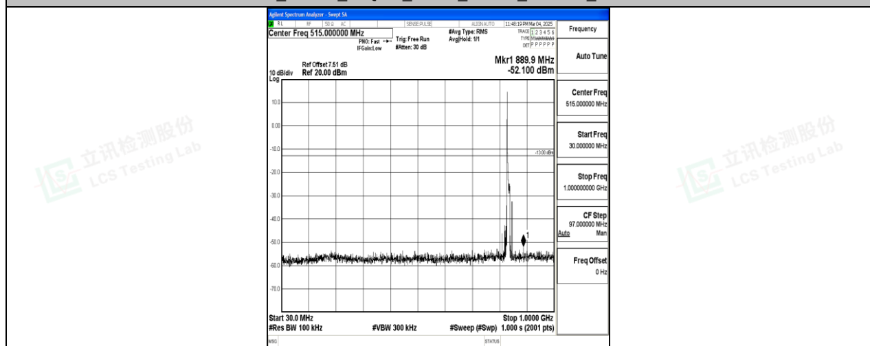
Band26_10MHz_16QAM_26915_1RB#0_30~1000_30~1000
