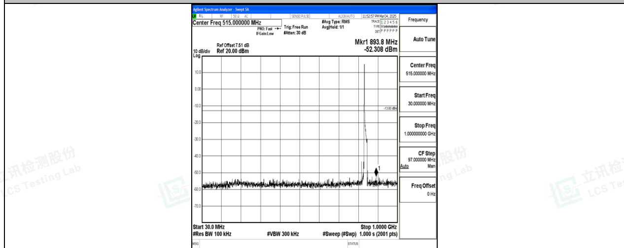
Band26_15MHz_QPSK_26965_1RB#0_30~1000_30~1000
