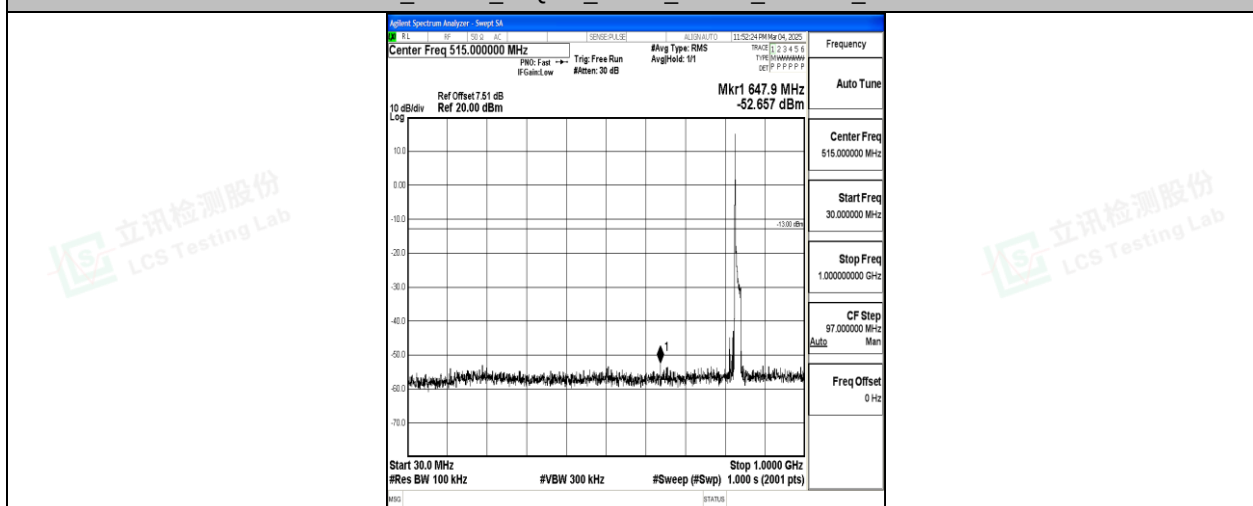
Band26_15MHz_16QAM_26915_1RB#0_30~1000_30~1000
