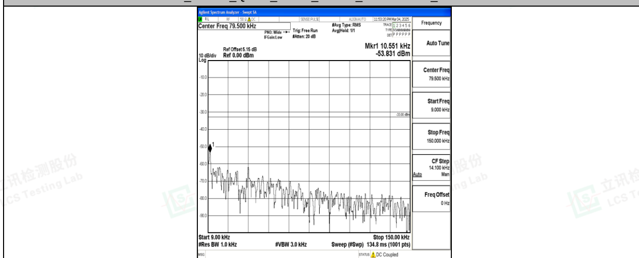
Band26_15MHz_16QAM_26965_1RB#0_0.009~0.15_0.009~0.15
