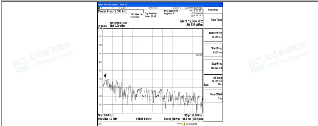
Band26_15MHz_QPSK_26965_1RB#0_0.009~0.15_0.009~0.15
