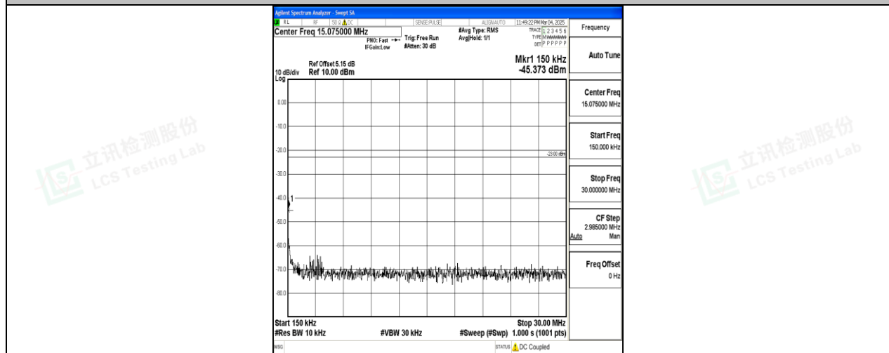
Band26_10MHz_16QAM_26990_1RB#0_0.15~30_0.15~30
