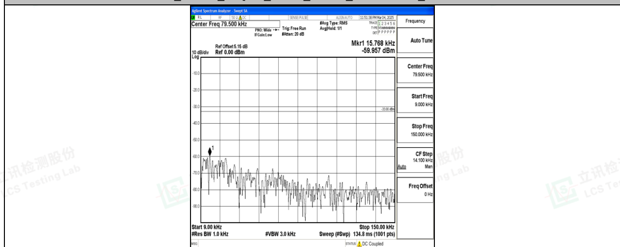
Band26_15MHz_QPSK_26915_1RB#0_0.009~0.15_0.009~0.15
