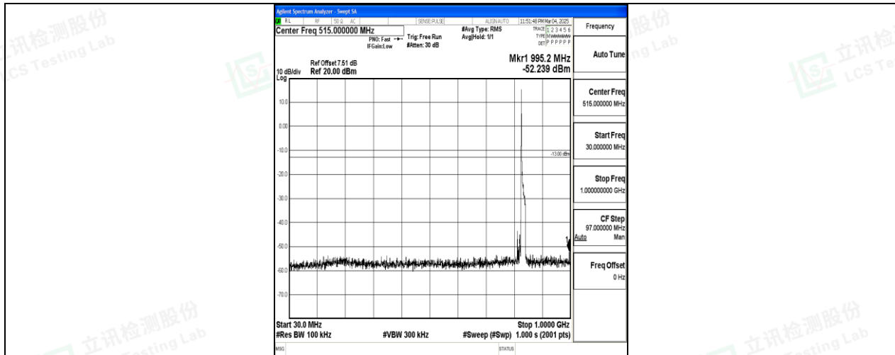
Band26_15MHz_QPSK_26915_1RB#0_30~1000_30~1000
