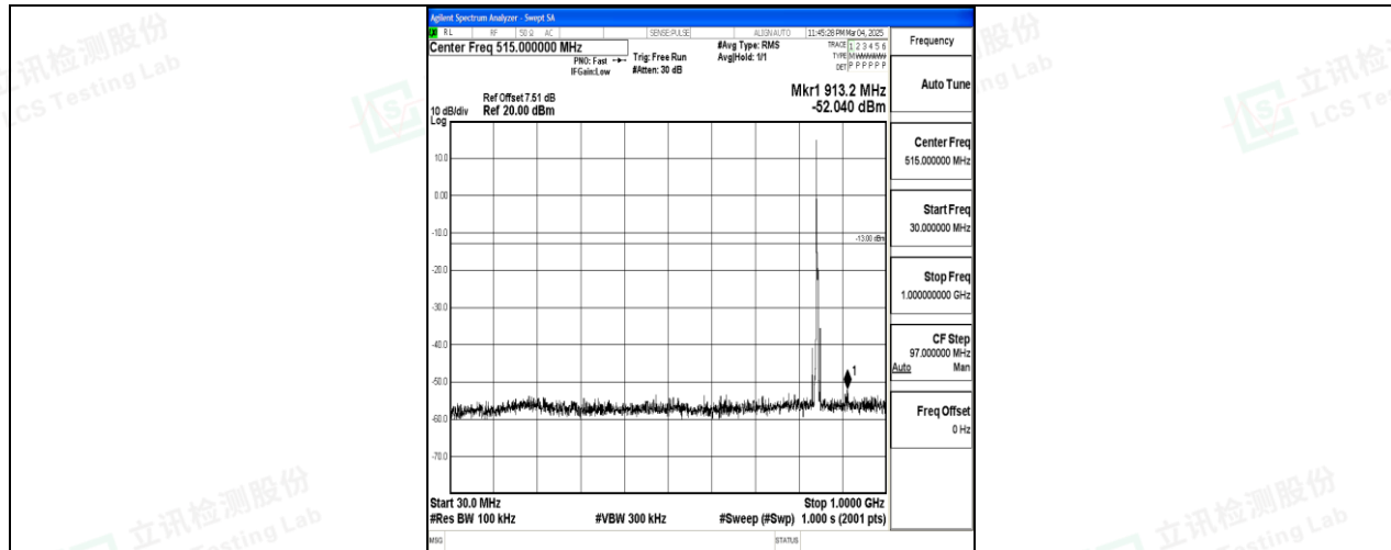
Band26_5MHz_16QAM_27015_1RB#0_30~1000_30~1000
