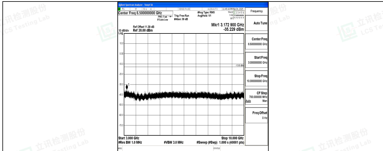
Band26_5MHz_QPSK_27015_1RB#0_3000~10000_3000~10000
