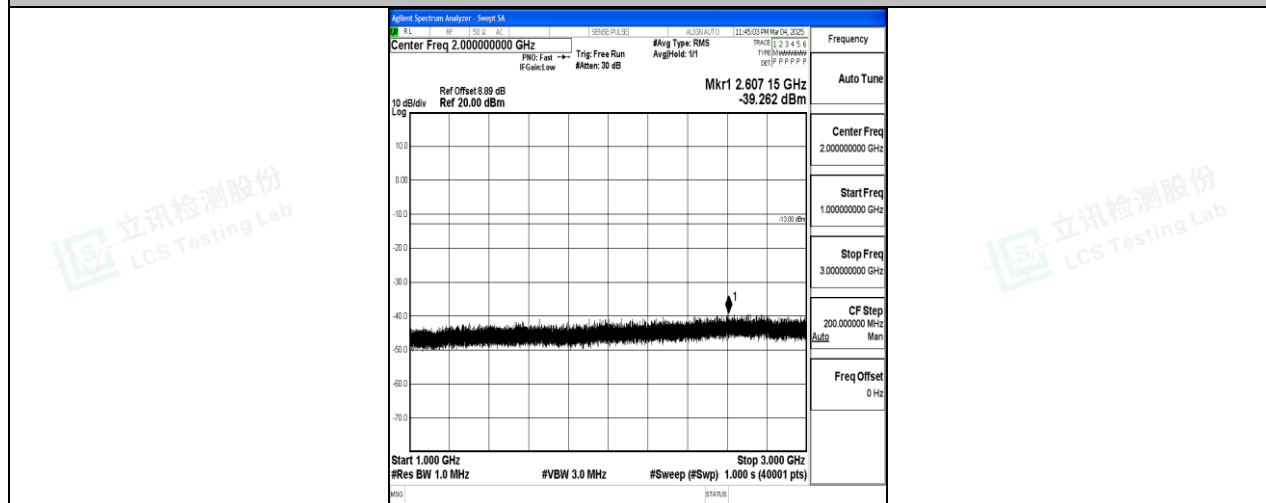
Band26_5MHz_QPSK_27015_1RB#0_1000~3000_1000~3000
