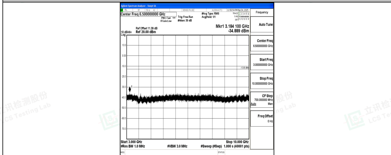
Band26_15MHz_QPSK_26865_1RB#0_3000~10000_3000~10000
