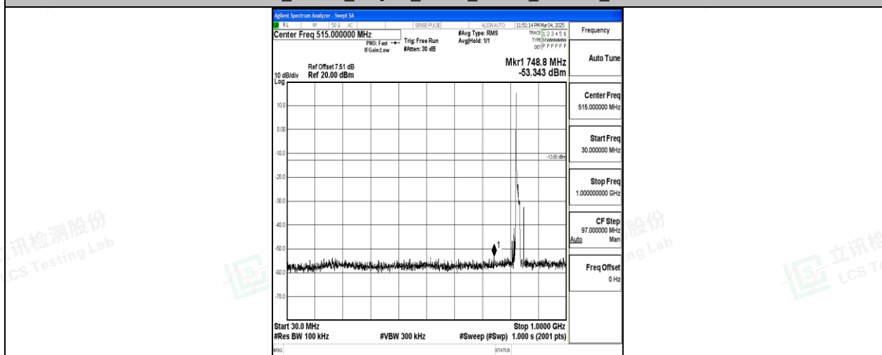
Band26_15MHz_16QAM_26865_1RB#0_30~1000_30~1000
