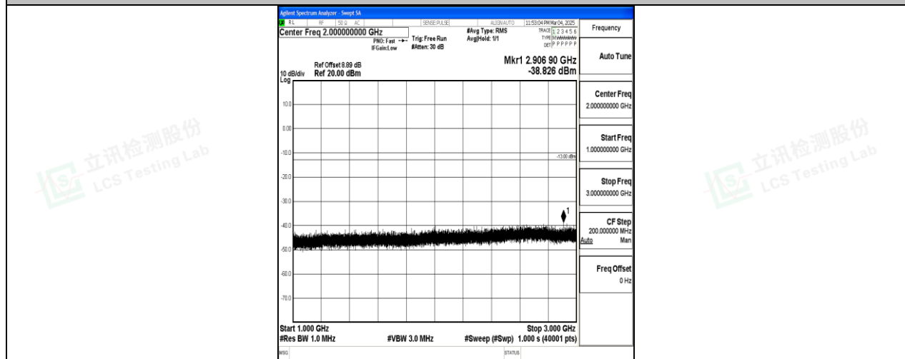
Band26_15MHz_QPSK_26965_1RB#0_1000~3000_1000~3000
