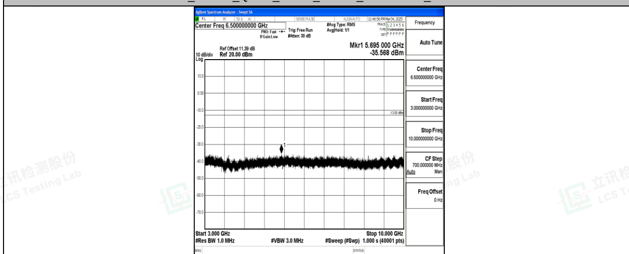
Band26_10MHz_QPSK_26840_1RB#0_3000~10000_3000~10000
