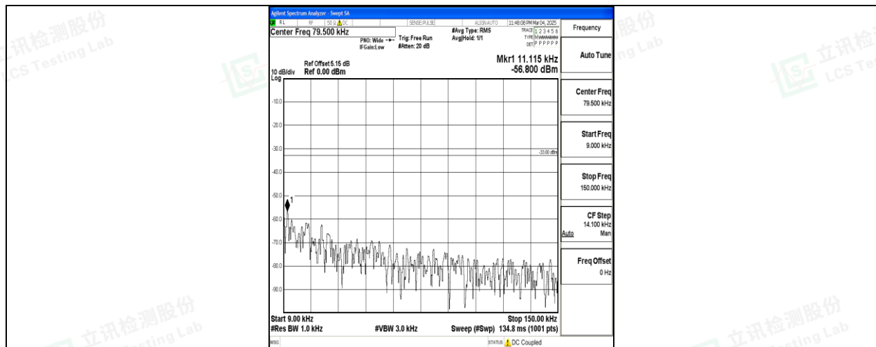
Band26_10MHz_16QAM_26915_1RB#0_0.009~0.15_0.009~0.15
