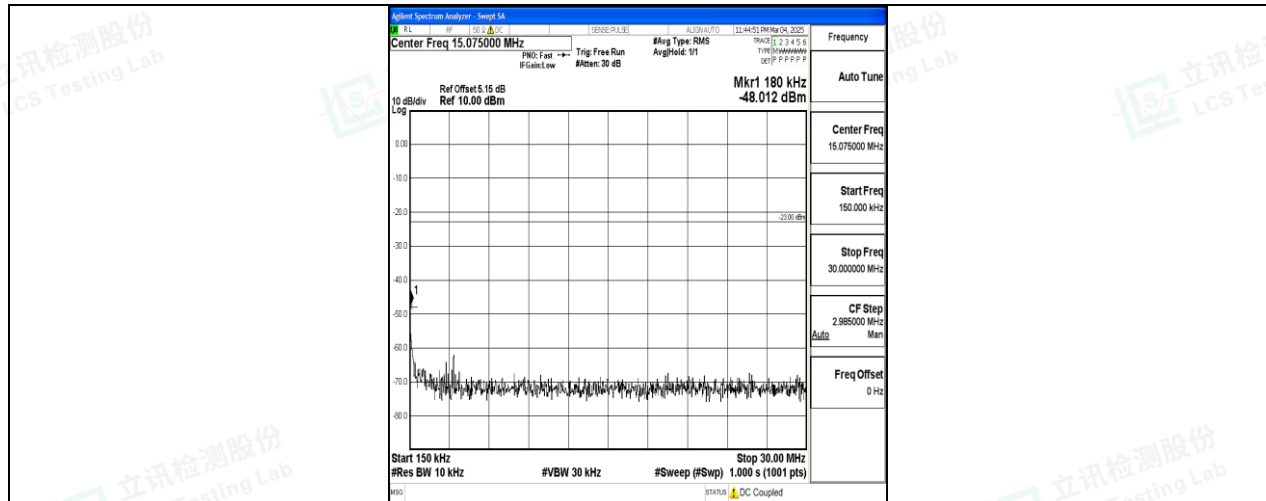
Band26_5MHz_QPSK_27015_1RB#0_0.15~30_0.15~30
