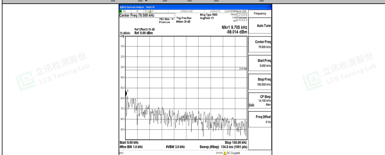
Band26_10MHz_16QAM_26840_1RB#0_0.009~0.15_0.009~0.15
