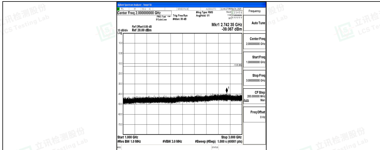
Band26_5MHz_16QAM_26915_1RB#0_1000~3000_1000~3000
