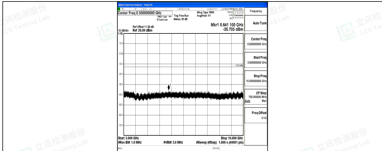
Band26_10MHz_QPSK_26990_1RB#0_3000~10000_3000~10000
