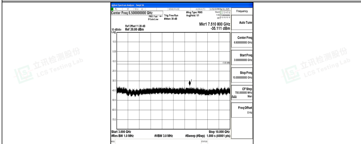
Band26_15MHz_QPSK_26915_1RB#0_3000~10000_3000~10000
