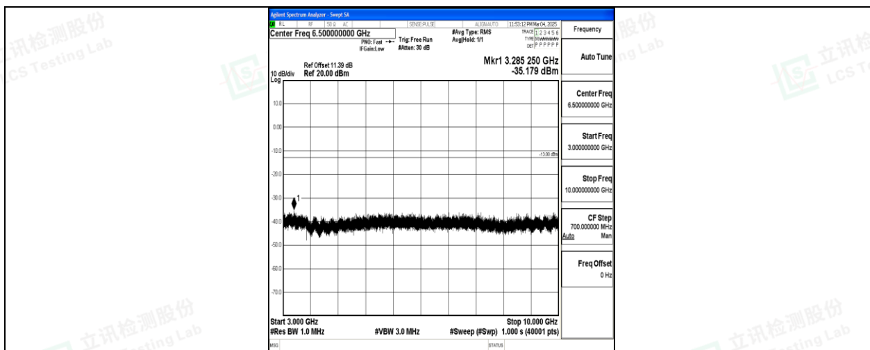
Band26_15MHz_QPSK_26965_1RB#0_3000~10000_3000~10000
