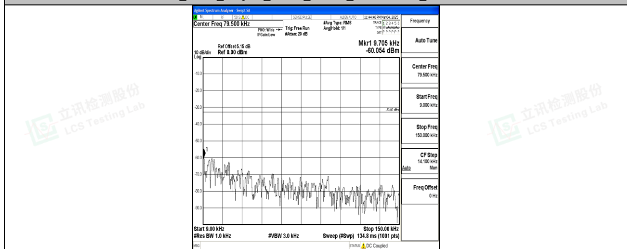
Band26_5MHz_QPSK_27015_1RB#0_0.009~0.15_0.009~0.15
