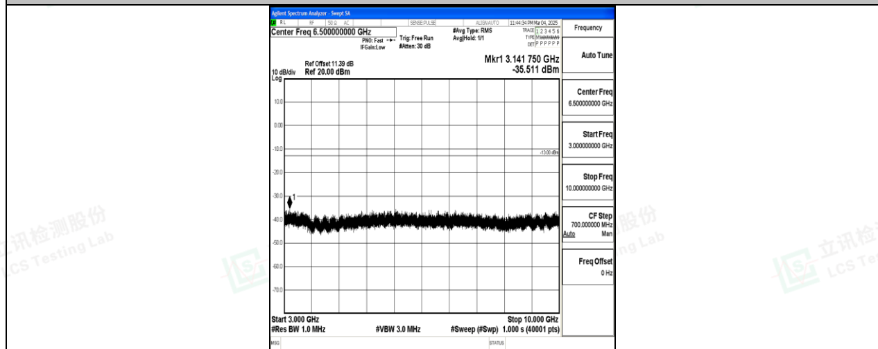
Band26_5MHz_16QAM_26915_1RB#0_3000~10000_3000~10000
