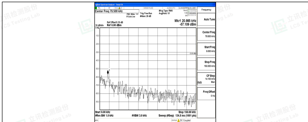
Band26_5MHz_16QAM_26915_1RB#0_0.009~0.15_0.009~0.15
