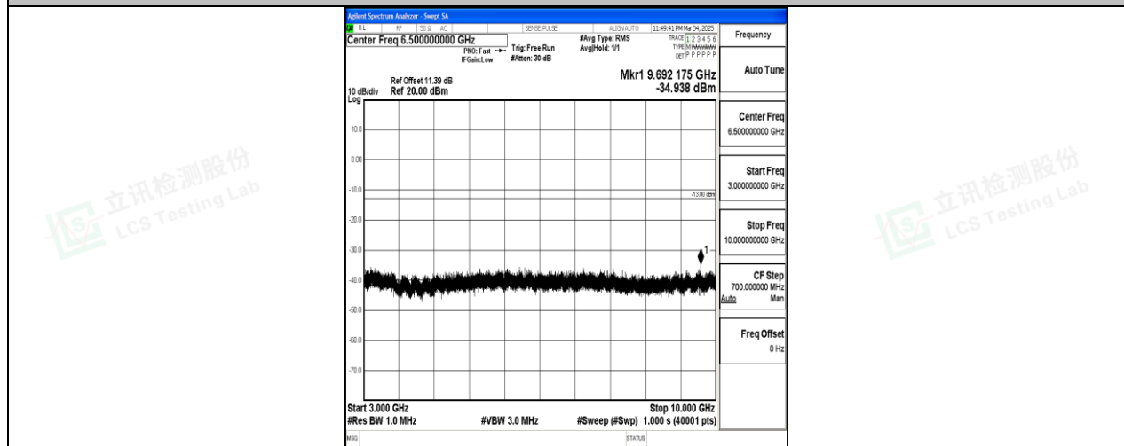
Band26_10MHz_16QAM_26990_1RB#0_3000~10000_3000~10000
