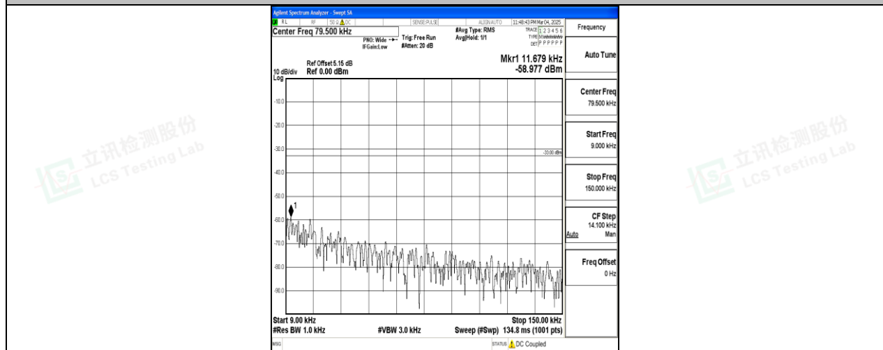
Band26_10MHz_QPSK_26990_1RB#0_0.009~0.15_0.009~0.15
