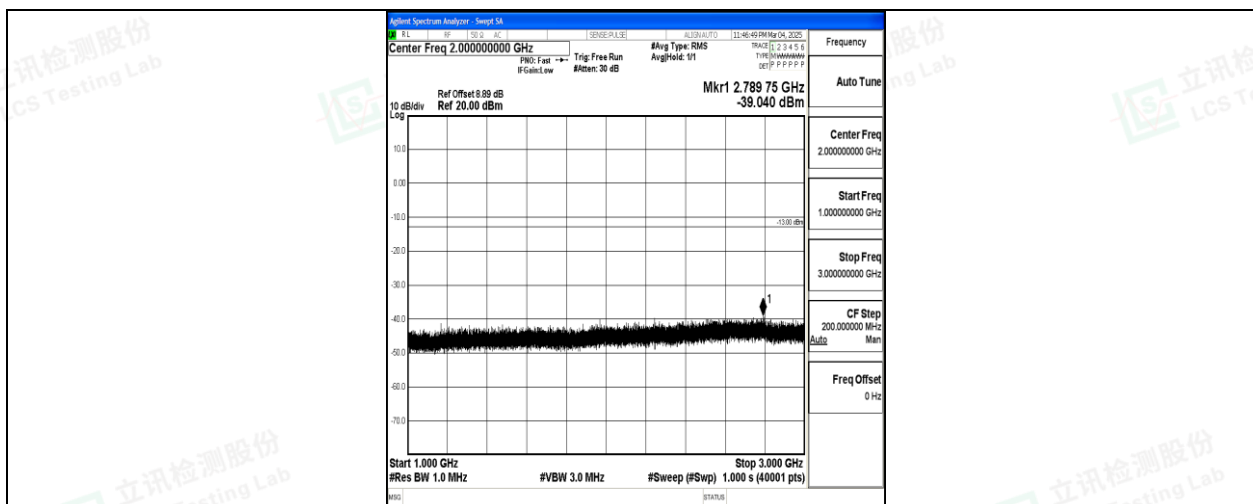
Band26_10MHz_QPSK_26840_1RB#0_1000~3000_1000~3000
