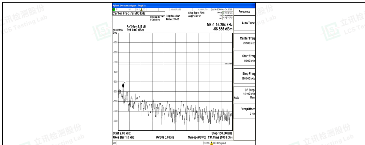
Band26_15MHz_QPSK_26865_1RB#0_0.009~0.15_0.009~0.15
