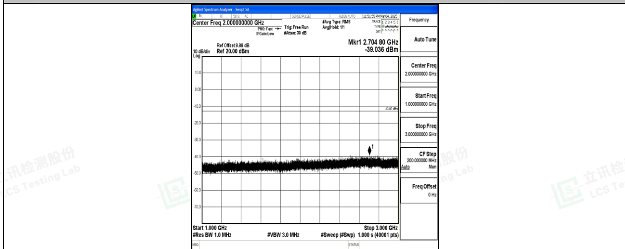
Band26_15MHz_QPSK_26915_1RB#0_1000~3000_1000~3000
