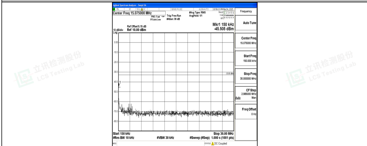
Band25_5MHz_16QAM_26065_1RB#0_0.15~30_0.15~30
