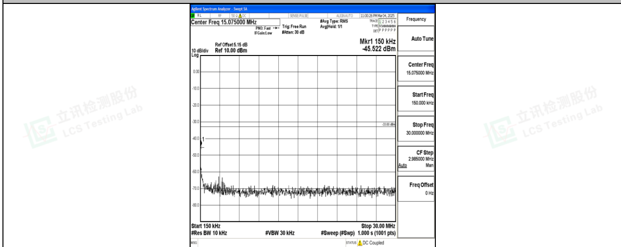
Band25_10MHz_16QAM_26090_1RB#0_0.15~30_0.15~30
