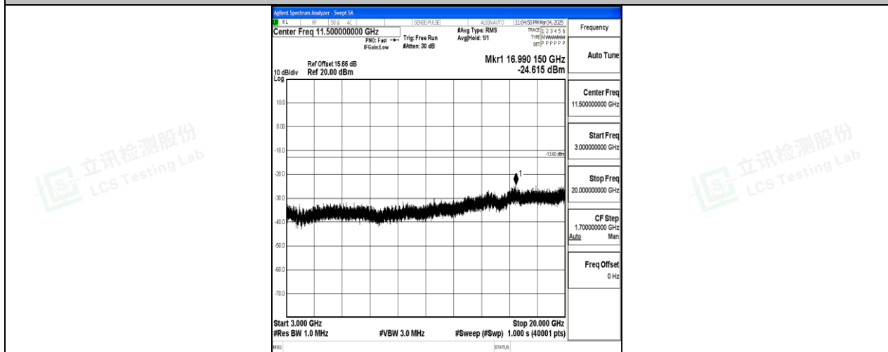
Band25_15MHz_16QAM_26115_1RB#0_3000~20000_3000~20000
