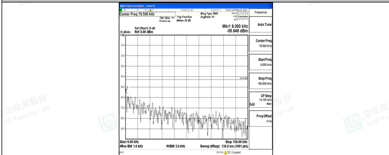
Band25_5MHz_16QAM_26065_1RB#0_0.009~0.15_0.009~0.15
