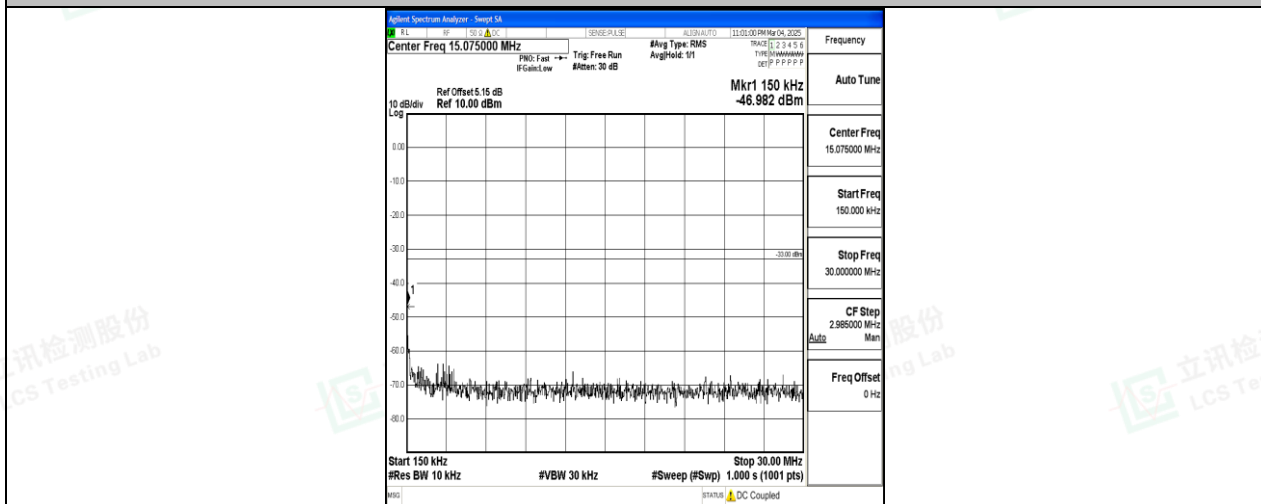
Band25_10MHz_QPSK_26365_1RB#0_0.15~30_0.15~30
