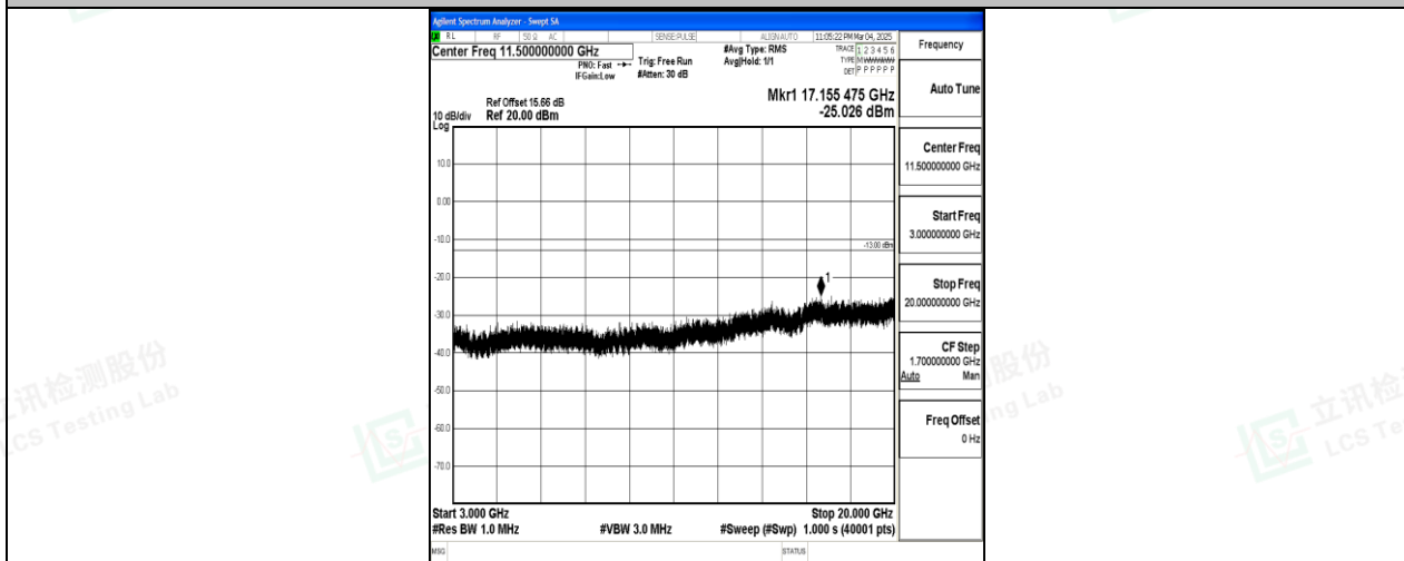
Band25_15MHz_QPSK_26365_1RB#0_3000~20000_3000~20000
