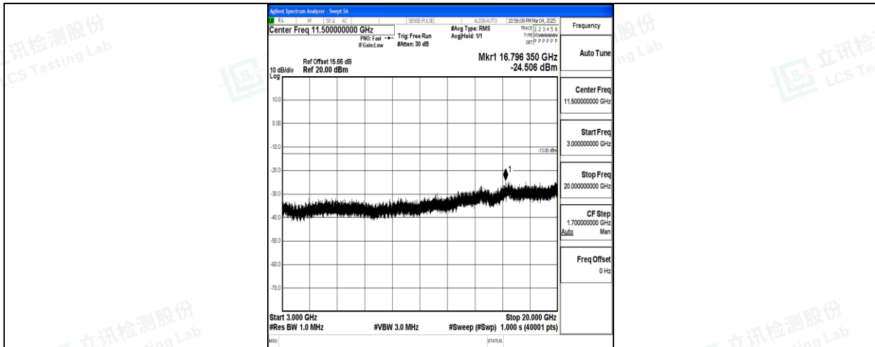
Band25_5MHz_QPSK_26065_1RB#0_3000~20000_3000~20000
