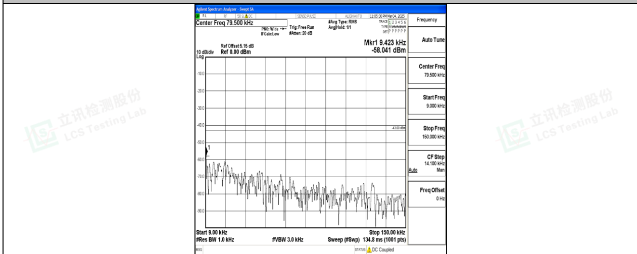
Band25_15MHz_16QAM_26365_1RB#0_0.009~0.15_0.009~0.15
