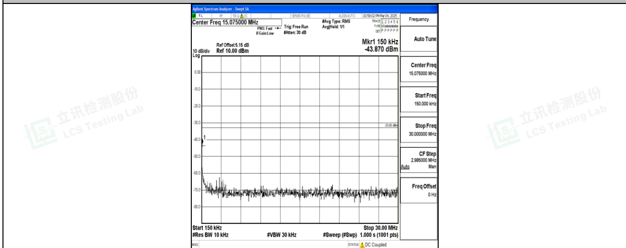
Band25_5MHz_QPSK_26665_1RB#0_0.15~30_0.15~30
