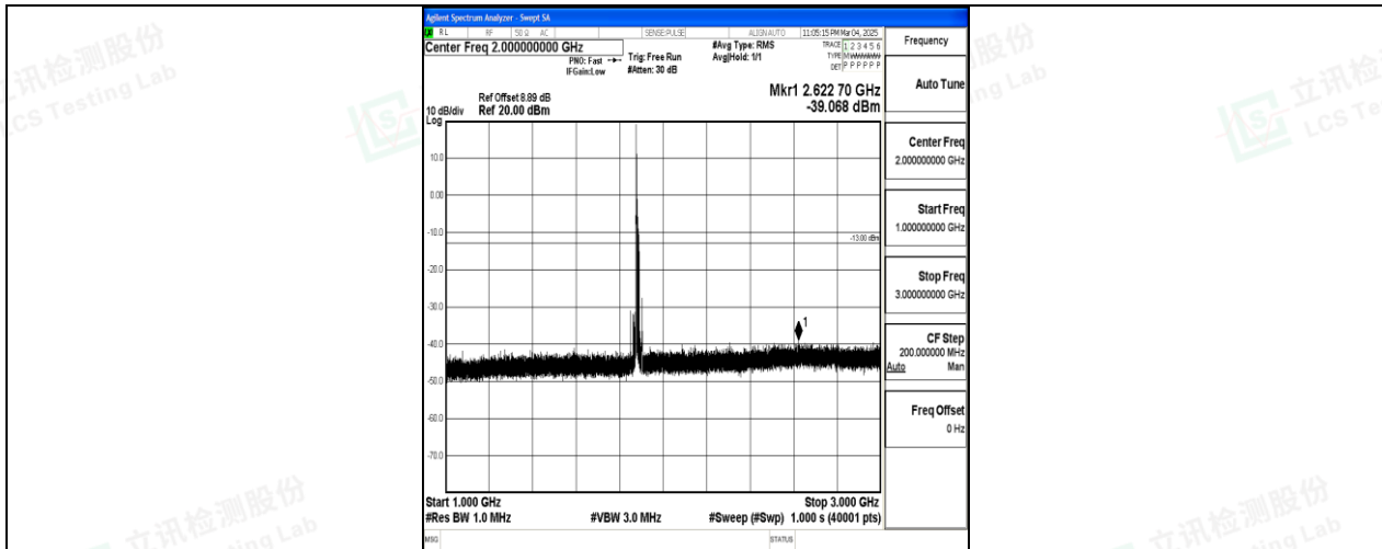
Band25_15MHz_QPSK_26365_1RB#0_1000~3000_1000~3000
