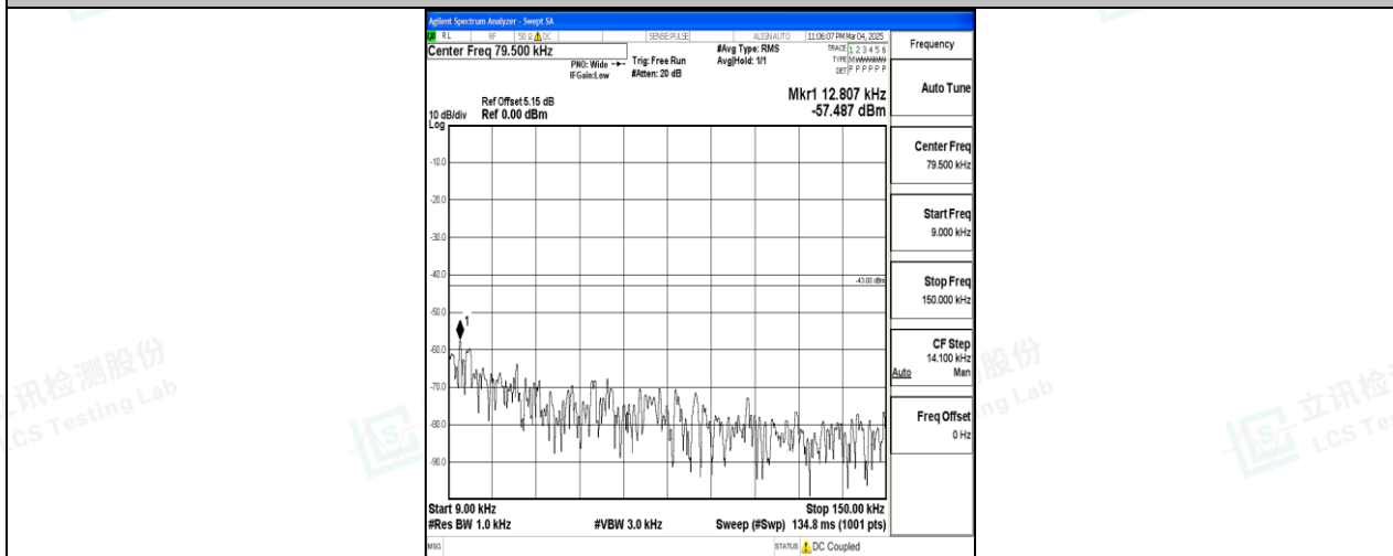
Band25_15MHz_QPSK_26615_1RB#0_0.009~0.15_0.009~0.15
