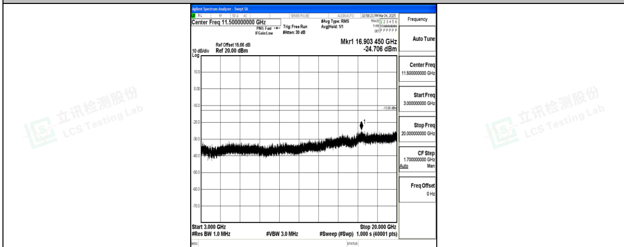
Band25_5MHz_QPSK_26665_1RB#0_3000~20000_3000~20000
