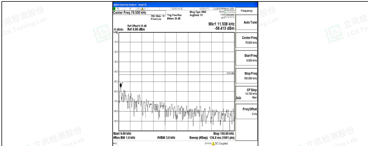
Band25_10MHz_QPSK_26365_1RB#0_0.009~0.15_0.009~0.15
