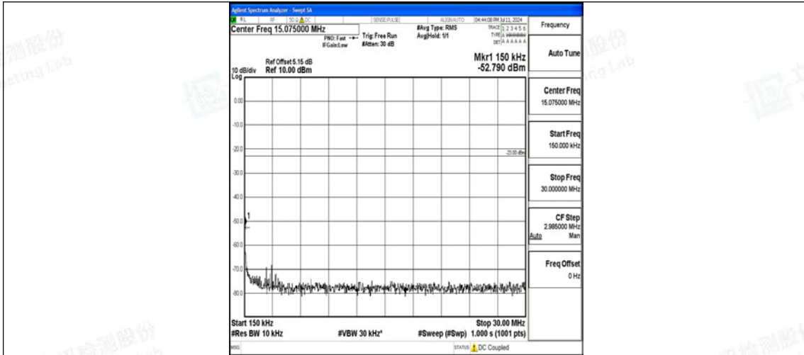
Band5_10MHz_QPSK_20600_1RB#0_0.15~30_0.15~30
