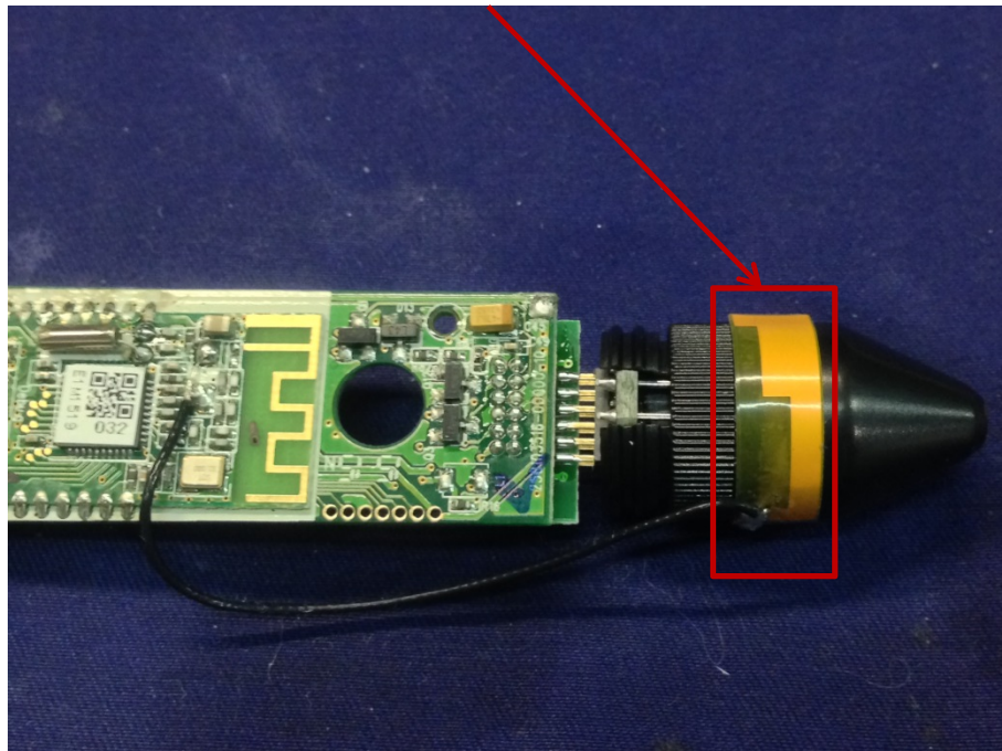
FPC Antenna
