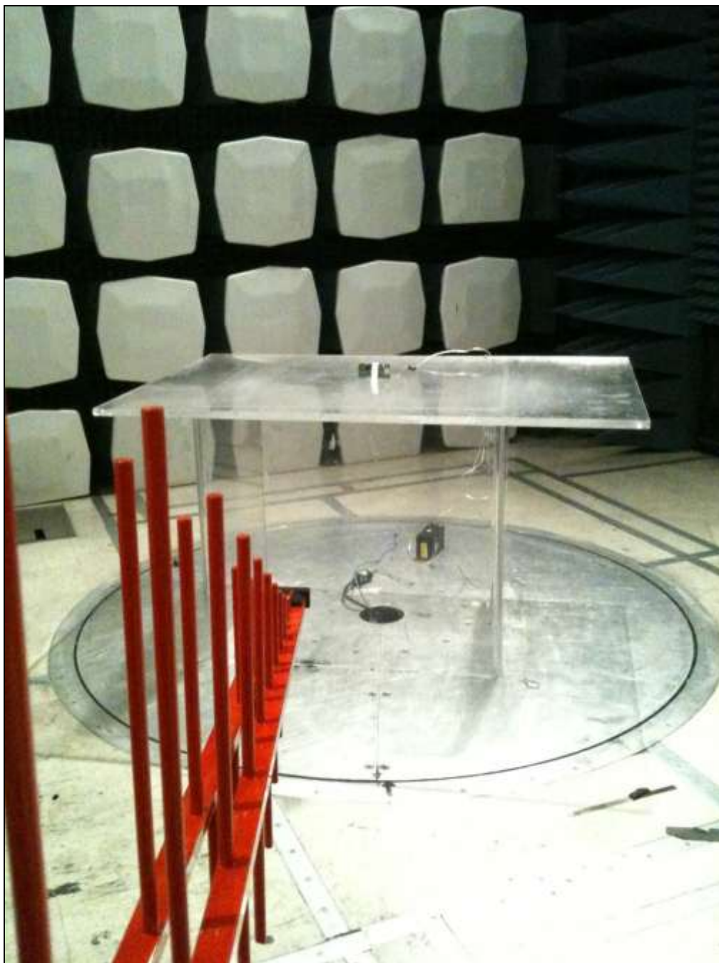
Photograph 2. Radiated Field Strength of Fundamental, Test Setup
