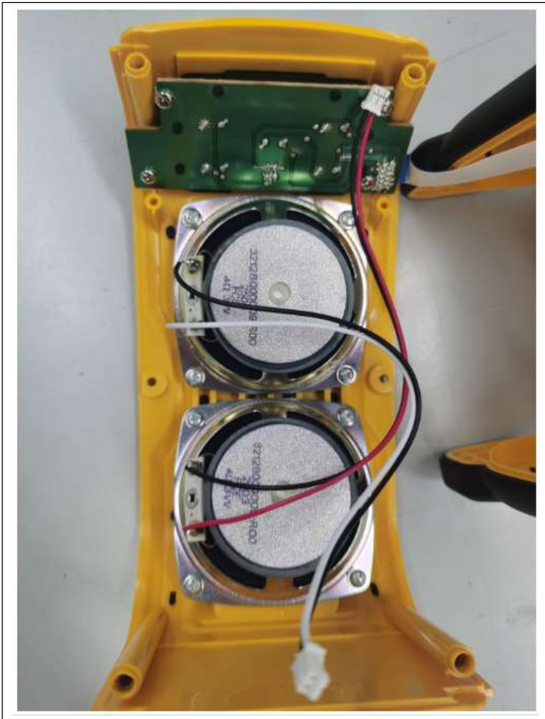
Front Enclosure Internal – UI PCA and Speaker Mounting
